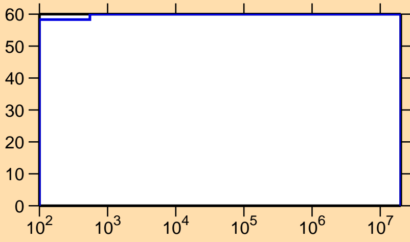
Delta \sigma/\sigma vs. E for ^{121}\text{Ce}(n,p)
