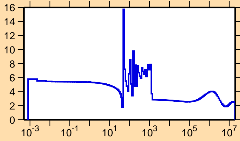
\sigma vs. E for ^{122}\text{Ce}(n,\text{el.})
