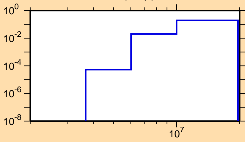
\sigma vs. E for ^{122}\text{Ce}(n,np)
