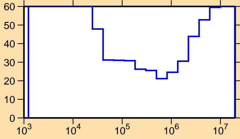
\Delta\sigma/\sigma vs. E for ^{122}\text{Ce}(n,p)
