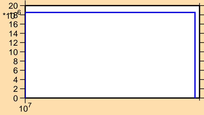
\sigma vs. E for ^{122}\text{Ce}(n,2n)
