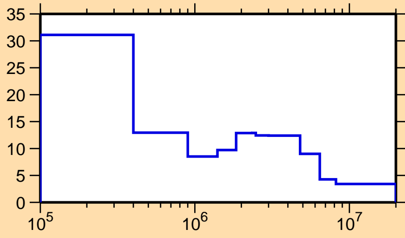
\Delta\sigma/\sigma vs. E for ^{122}\text{Ce}(n,\text{tot.})
