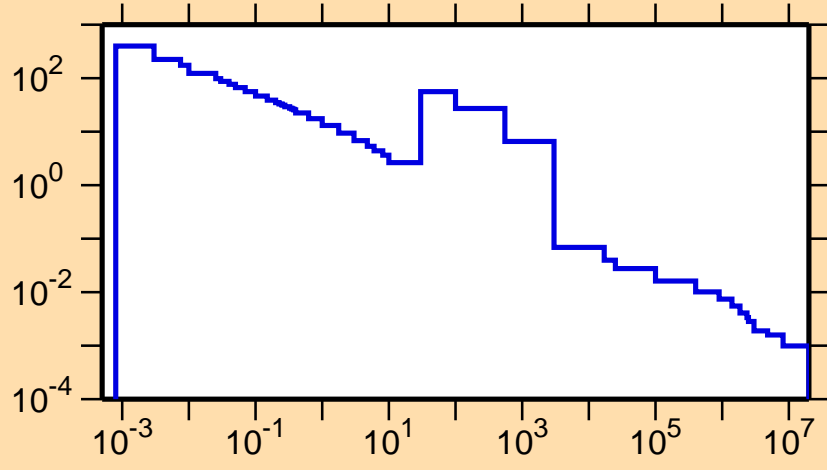
\sigma vs. E for ^{122}\text{Ce}(n,\gamma)
