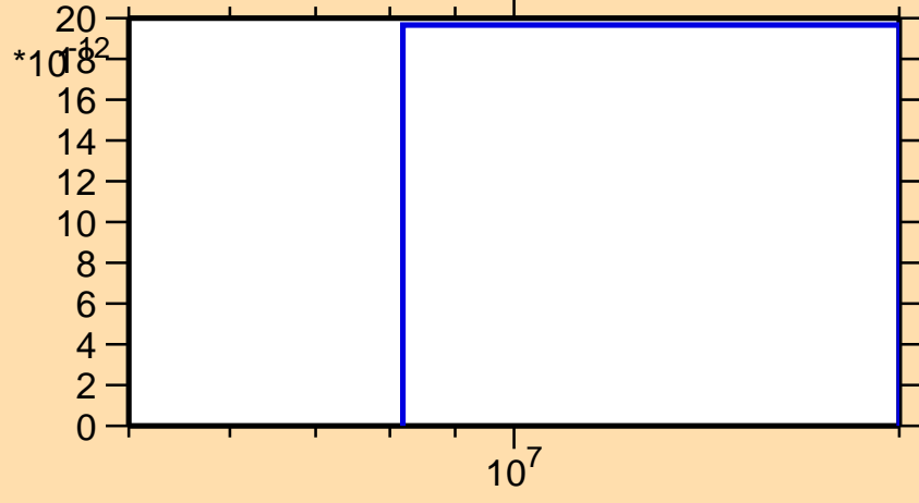
\sigma vs. E for ^{122}\text{Ce}(\text{mt } 34)
