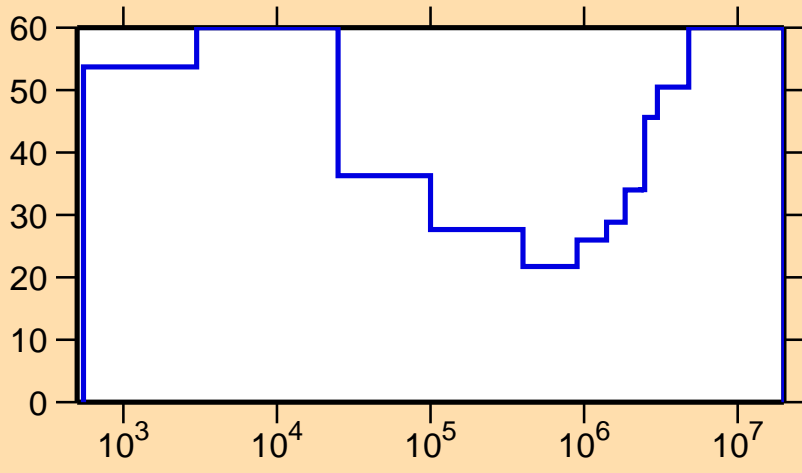
\Delta\sigma/\sigma vs. E for ^{122}\text{Ce}(n,p)
