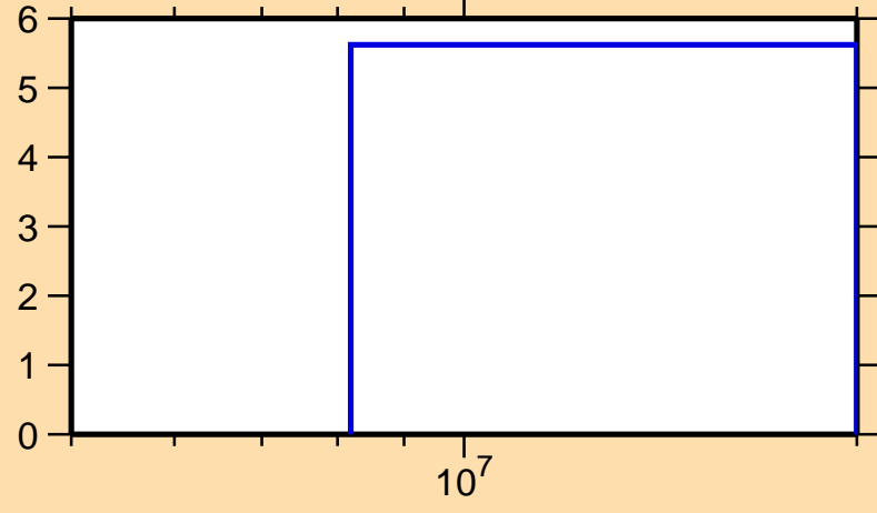
\Delta\sigma/\sigma vs. E for ^{122}\text{Ce}(n,\text{el.})
