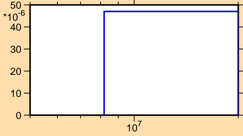
\sigma vs. E for ^{122}\text{Ce}(n,t)
