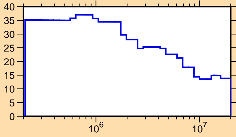
\Delta\sigma/\sigma vs. E for ^{123}\text{Ce}(n,n\text{onel.})
