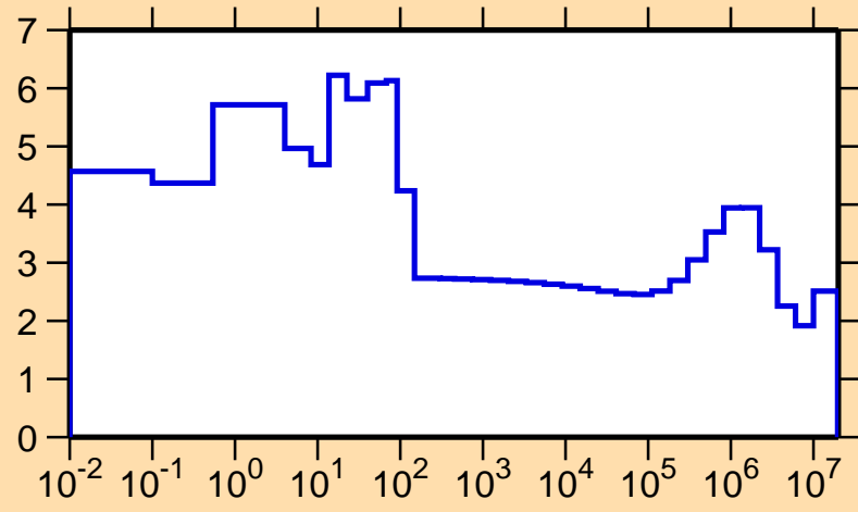
\sigma vs. E for ^{123}\text{Ce}(n,\text{el.})
