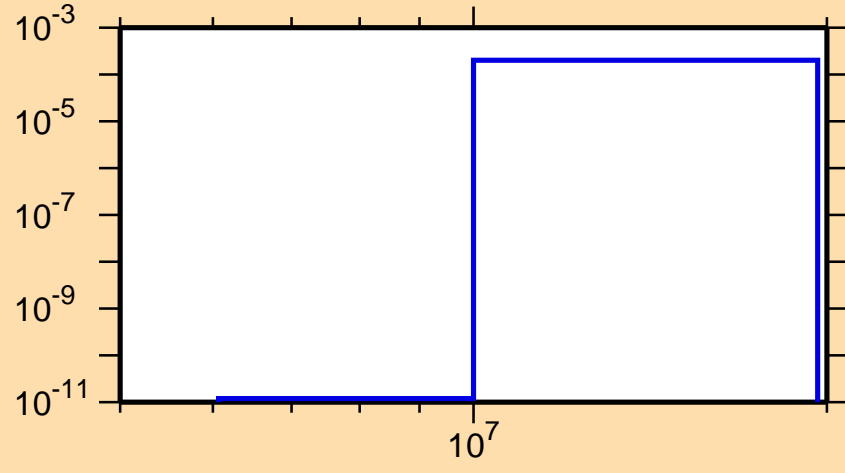
\sigma vs. E for ^{123}\text{Ce}(n,t)
