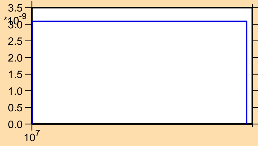
\sigma vs. E for ^{123}\text{Ce} (mt 34)
