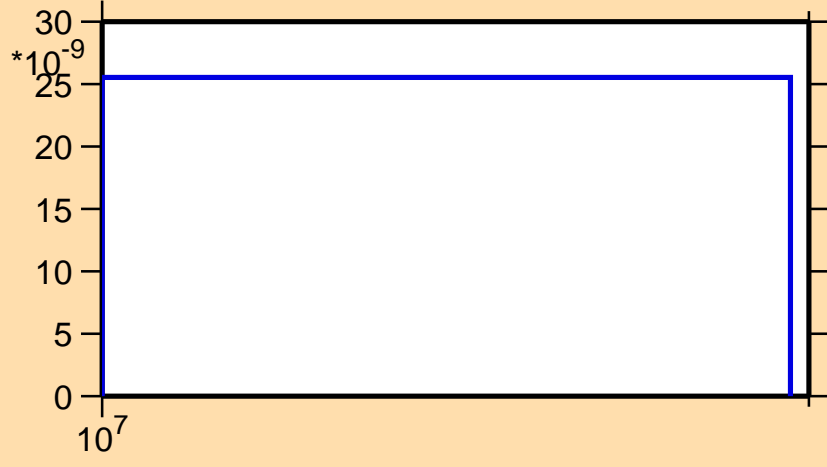
\sigma vs. E for ^{123}\text{Ce}(n,2n\alpha)
