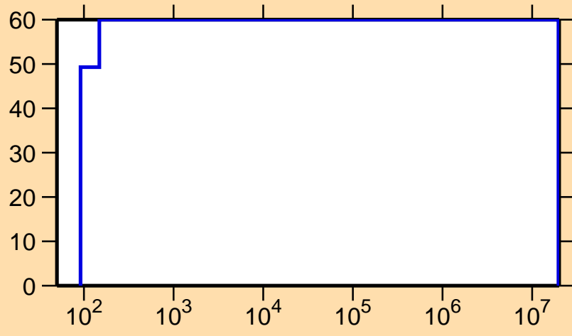
\Delta\sigma/\sigma vs. E for ^{123}\text{Ce}(n,p)
