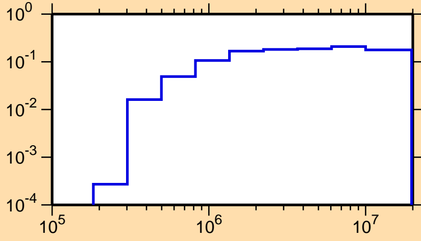
\sigma vs. E for ^{123}\text{Ce}(n,\text{inel.})
