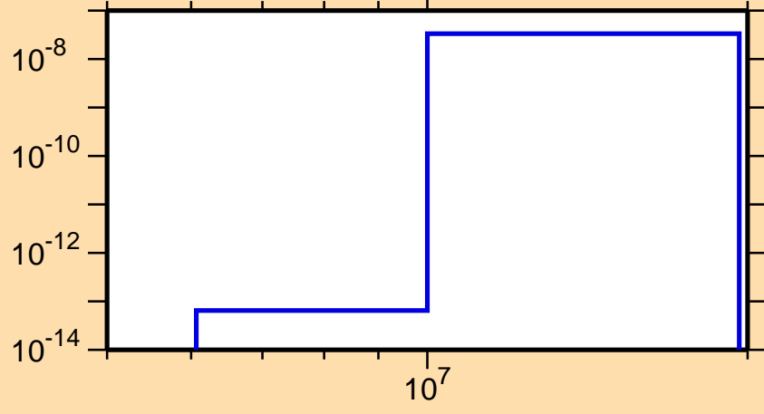
\sigma vs. E for ^{123}\text{Ce}(\text{mt117})
