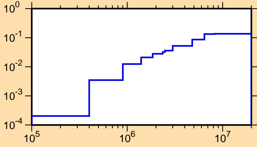
\sigma vs. E for ^{123}\text{Ce}(n,n\text{cont.})
