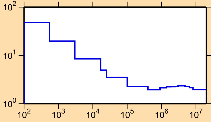
\sigma vs. E for ^{123}\text{Ce}(n,\text{nonel.})
