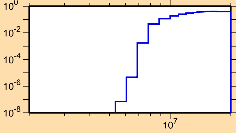
\sigma vs. E for ^{124}\text{Ce}(n,np)
