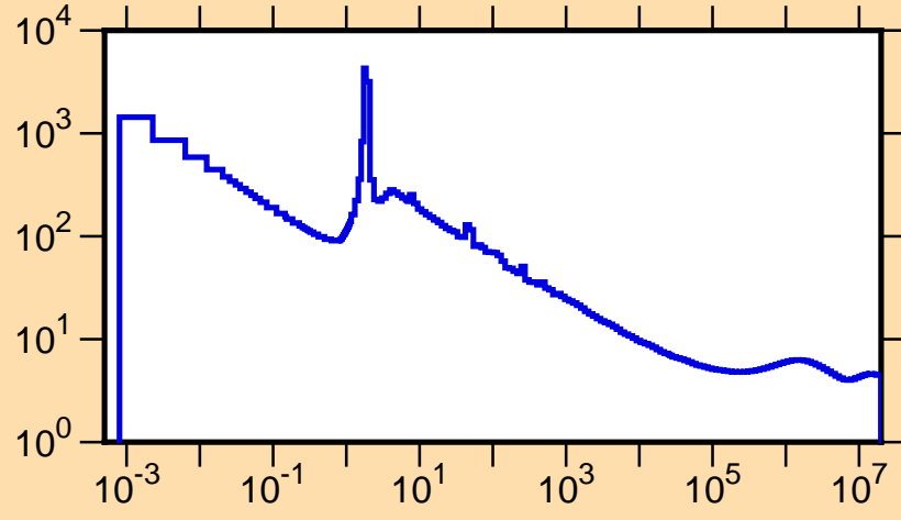
\sigma vs. E for ^{124}\text{Ce}(n,\text{tot.})
