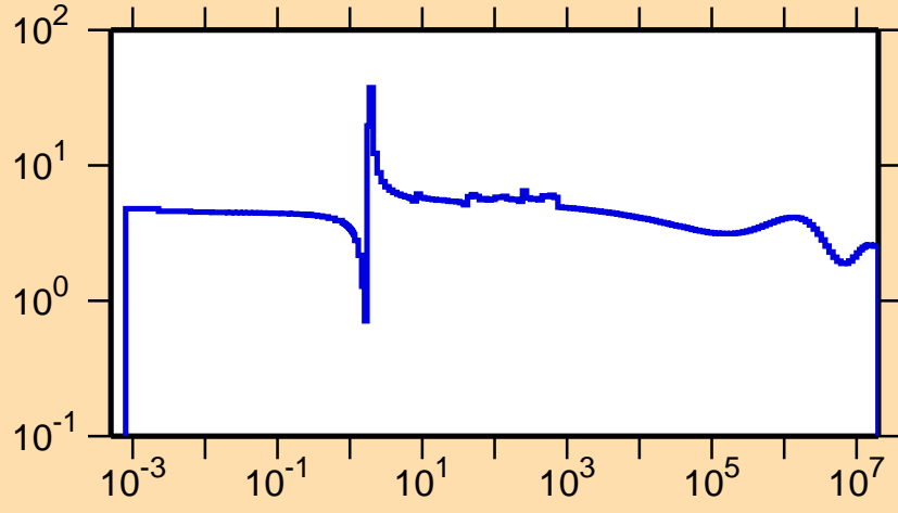
\sigma vs. E for ^{124}\text{Ce}(n,\text{el.})
