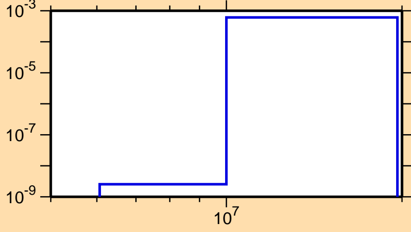
\sigma vs. E for ^{124}\text{Ce}(n,\text{pd})
