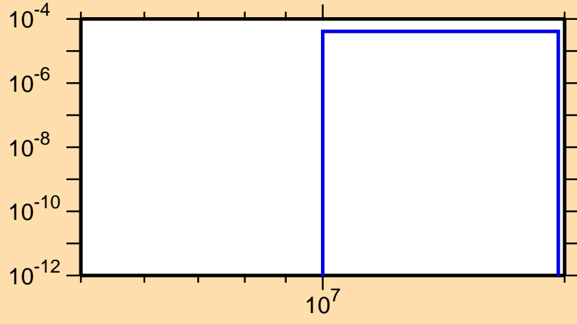
\sigma vs. E for ^{124}\text{Ce}(n,t)
