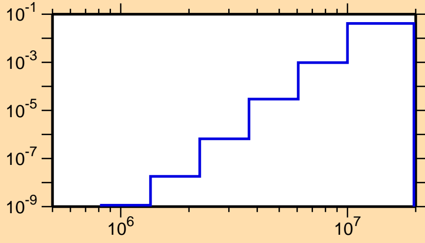
\sigma vs. E for ^{124}\text{Ce}(n,p\alpha)
