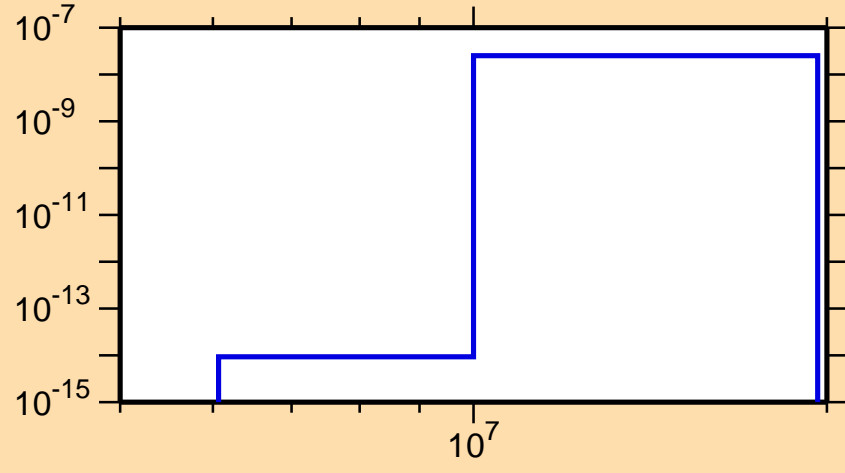
\sigma vs. E for ^{124}\text{Ce}(\text{mt117})
