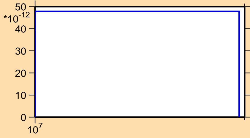
\sigma vs. E for ^{124}\text{Ce}(n,\text{nd})
