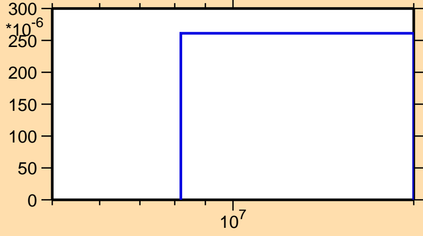
\sigma vs. E for ^{124}\text{Ce}(n,2n)
