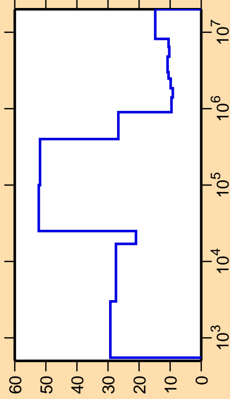
\Delta\sigma/\sigma vs. E for ^{124}\text{Ce}(n,\text{nonel.})
