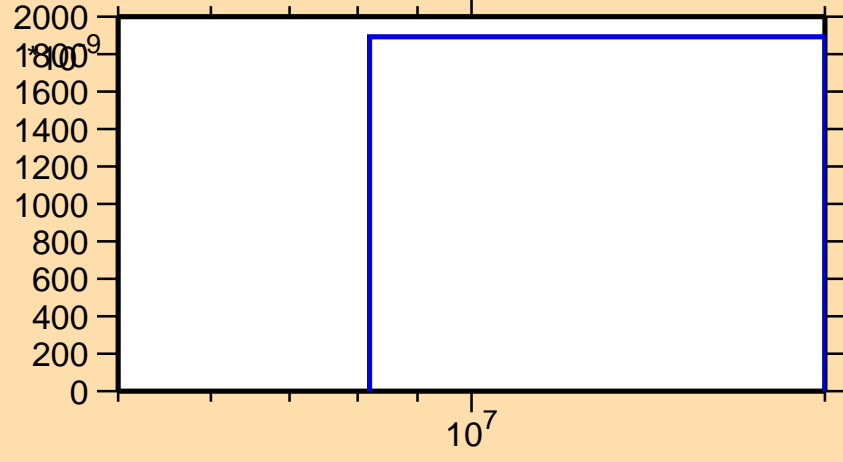
\sigma vs. E for ^{124}\text{Ce}(\text{mt } 45)
