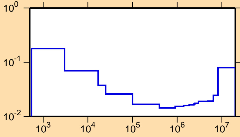
\sigma vs. E for ^{124}\text{Ce}(n,\alpha)
