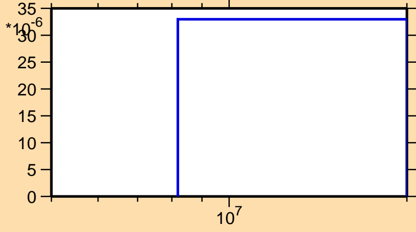
\sigma vs. E for ^{124}\text{Ce}(n,t)
