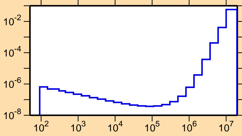
\sigma vs. E for ^{125}\text{Ce}(n,p\alpha)
