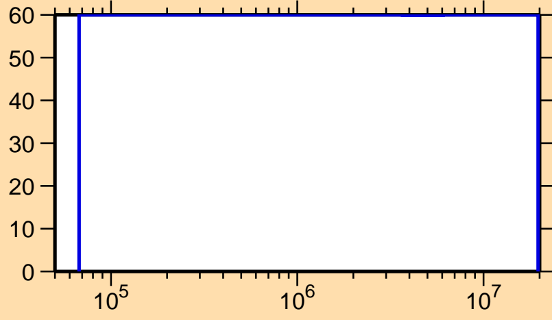
\Delta\sigma/\sigma vs. E for ^{125}\text{Ce}(n,n_1)
