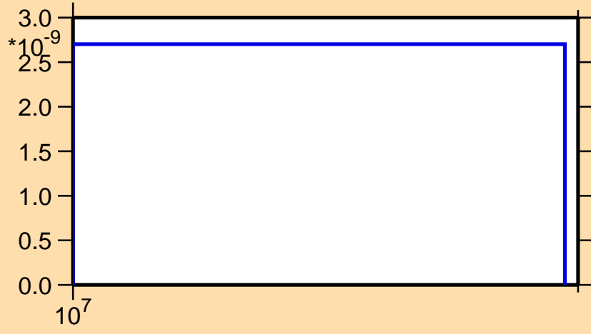
\sigma vs. E for ^{125}\text{Ce} (mt 34)
