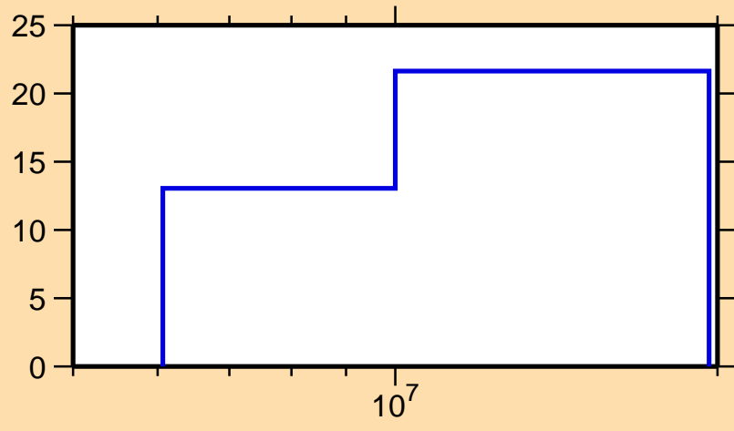
\Delta\sigma/\sigma vs. E for ^{125}\text{Ce}(n,\text{nonel.})
