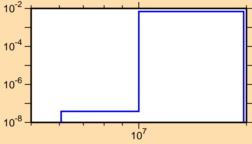
\sigma vs. E for ^{125}\text{Ce}(n,2n)
