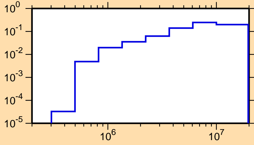
\sigma vs. E for ^{125}\text{Ce}(n,n\text{cont.})
