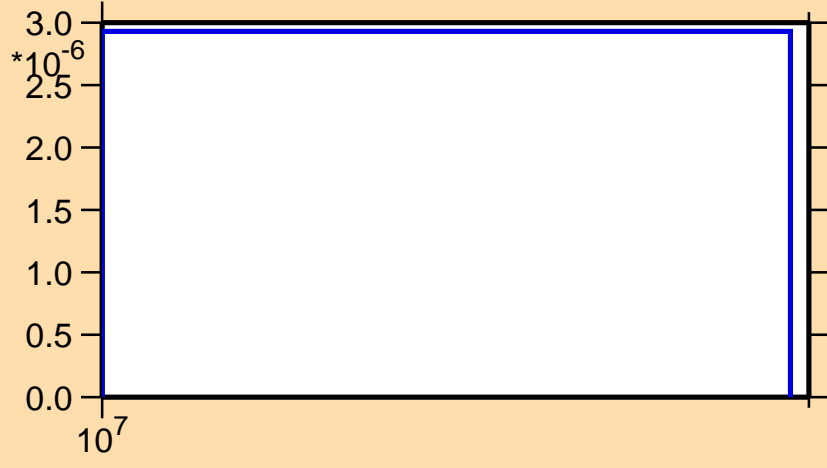
\sigma vs. E for ^{125}\text{Ce}(n,2np)
