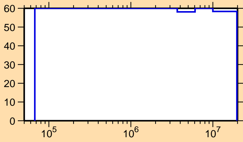
\Delta\sigma/\sigma vs. E for ^{125}\text{Ce}(n,\text{inel.})
