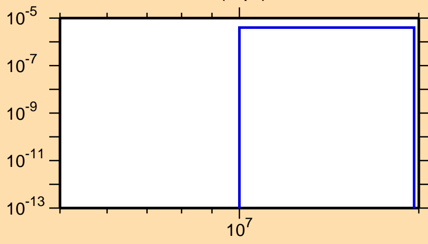
\sigma vs. E for ^{125}\text{Ce}(n,pt)
