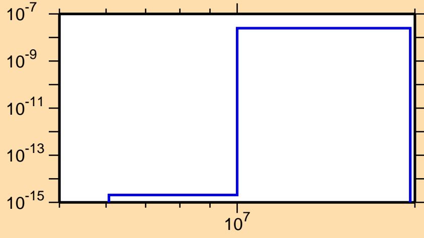
\sigma vs. E for ^{125}\text{Ce}(\text{mt117})
