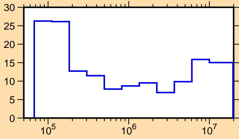
\Delta\sigma/\sigma vs. E for ^{125}\text{Ce}(n,\text{tot.})
