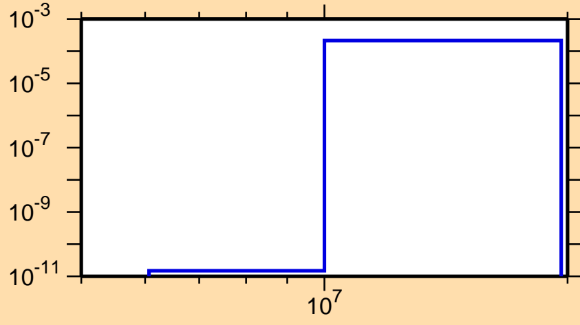
\sigma vs. E for ^{125}\text{Ce}(n,t)
