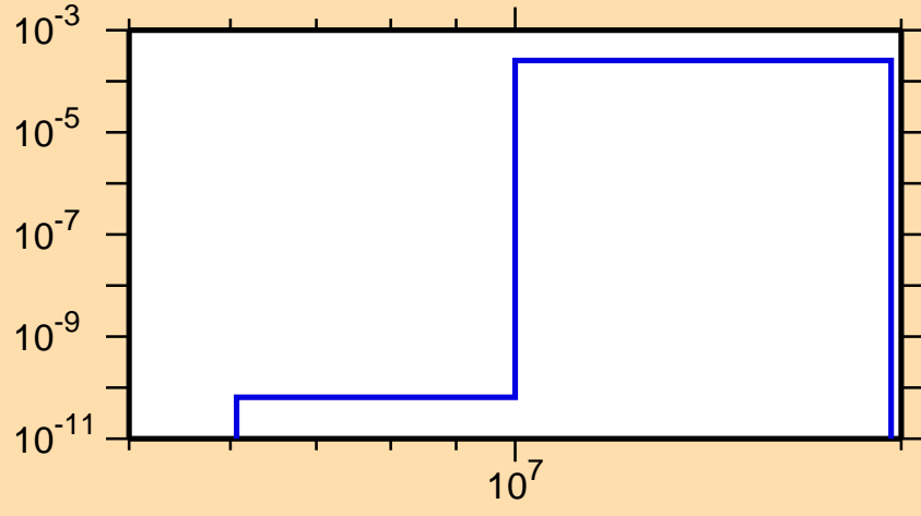
\sigma vs. E for ^{125}\text{Ce}(n,\text{pd})
