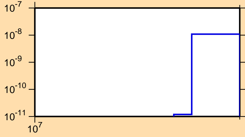
\sigma vs. E for ^{126}\text{Ce}(n,\text{nd})
