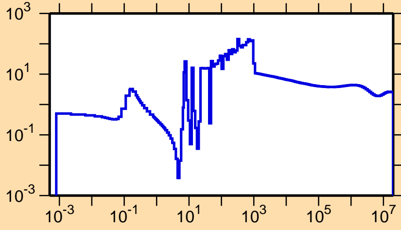
\sigma vs. E for ^{126}\text{Ce}(n,\text{el.})
