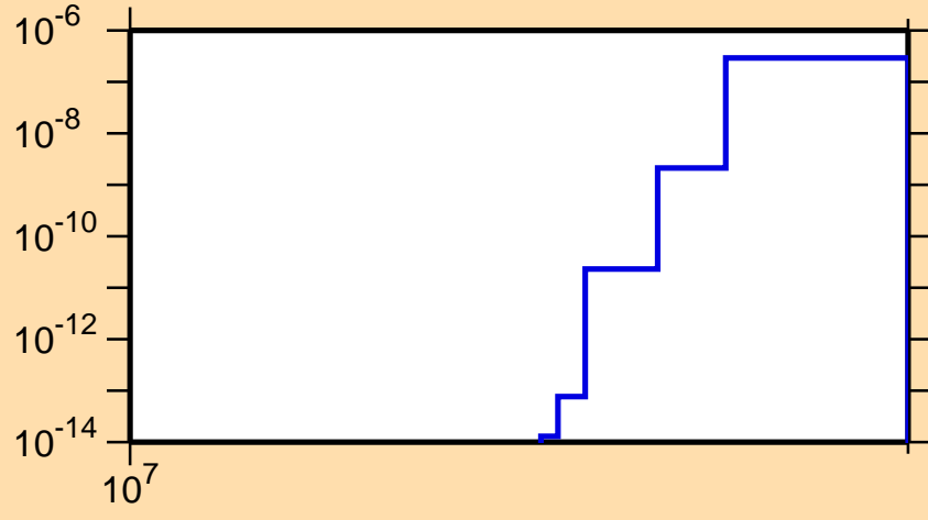
\sigma vs. E for ^{126}\text{Ce}(n,\text{pt})
