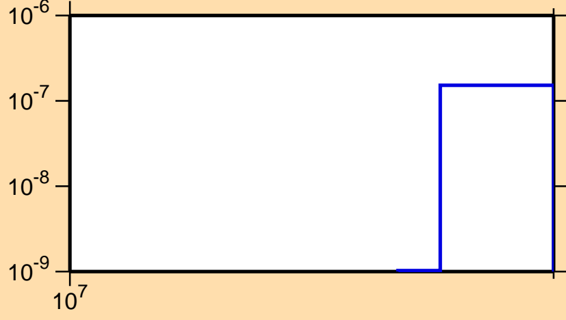
\sigma vs. E for ^{126}\text{Ce}(n,2n\alpha)
