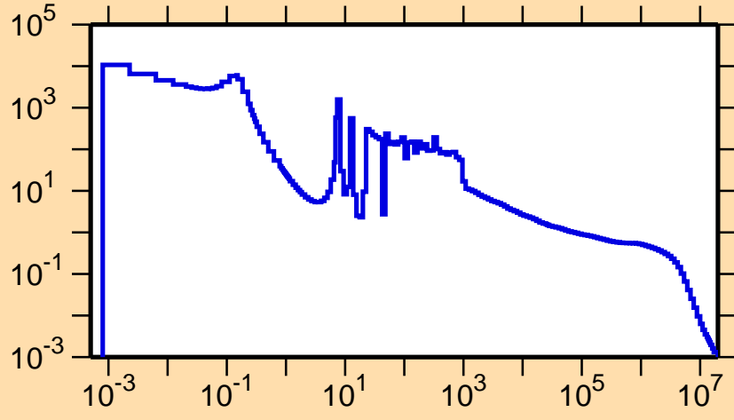
\sigma vs. E for ^{126}\text{Ce}(n,\gamma)
