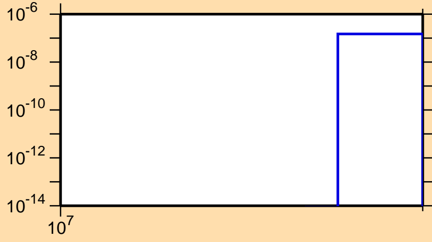
\sigma vs. E for ^{126}\text{Ce}(n,2np)
