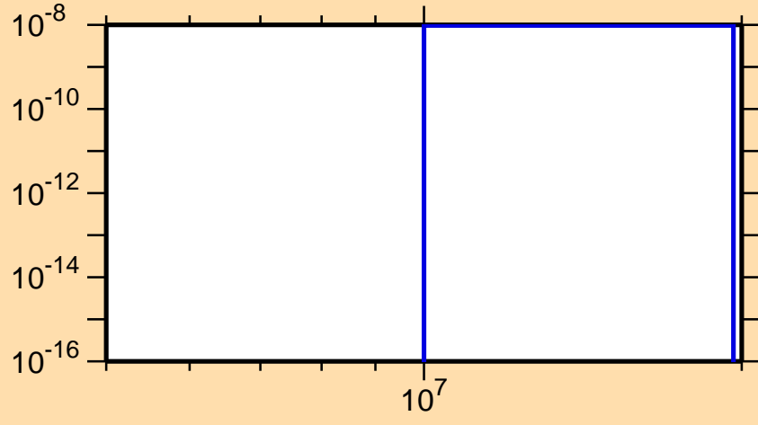
\sigma vs. E for ^{126}\text{Ce}(\text{mt117})
