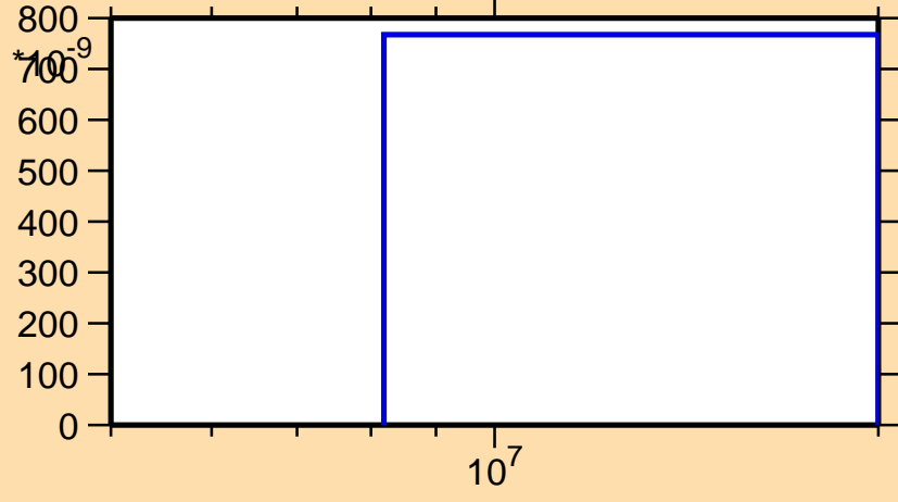
\sigma vs. E for ^{126}\text{Ce}(\text{mt } 45)
