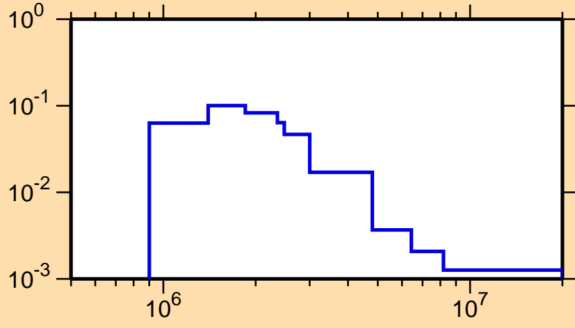
\sigma vs. E for ^{126}\text{Ce}(n,n_3)
