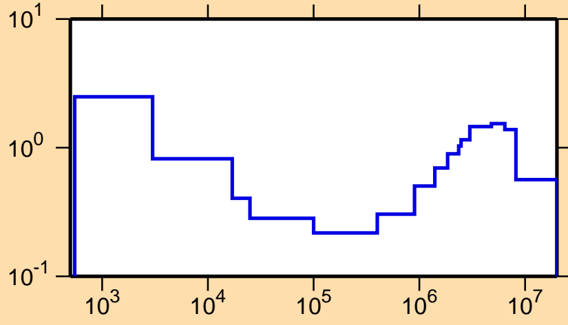
\sigma vs. E for ^{126}\text{Ce}(n,p)
