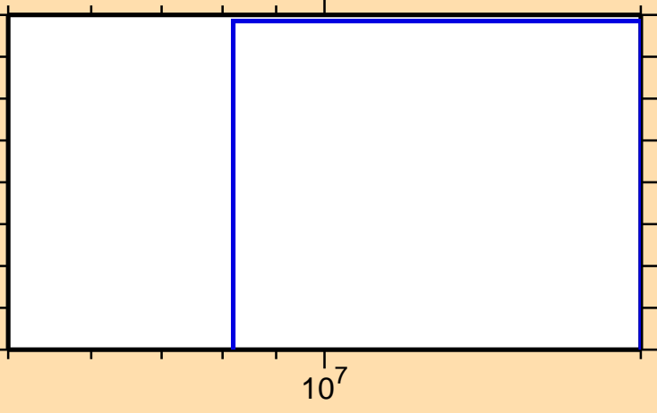
\sigma vs. E for ^{126}\text{Ce}(\text{mt117})
