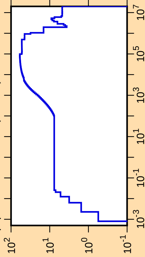
\Delta\mu/\mu vs. E for ^{127}\text{Ce}(\text{mt251})
