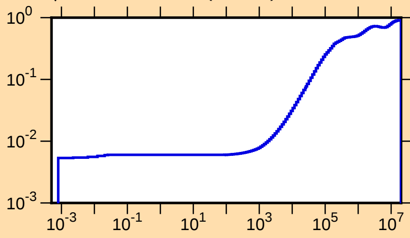
\mu vs. E for ^{127}\text{Ce}(\text{mt251})
