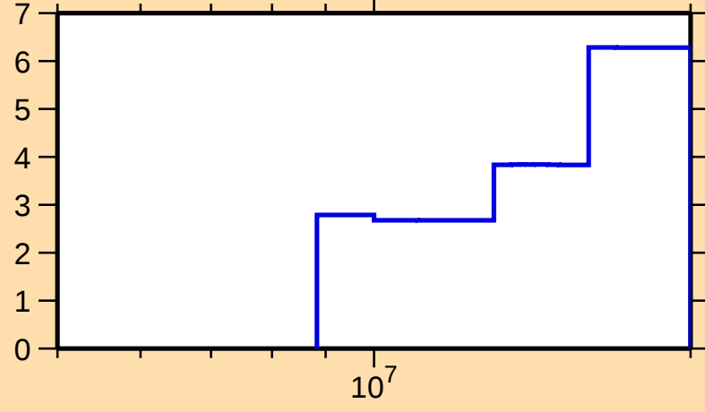
\Delta\sigma/\sigma vs. E for ^{127}\text{Ce}(n,\text{tot.})
