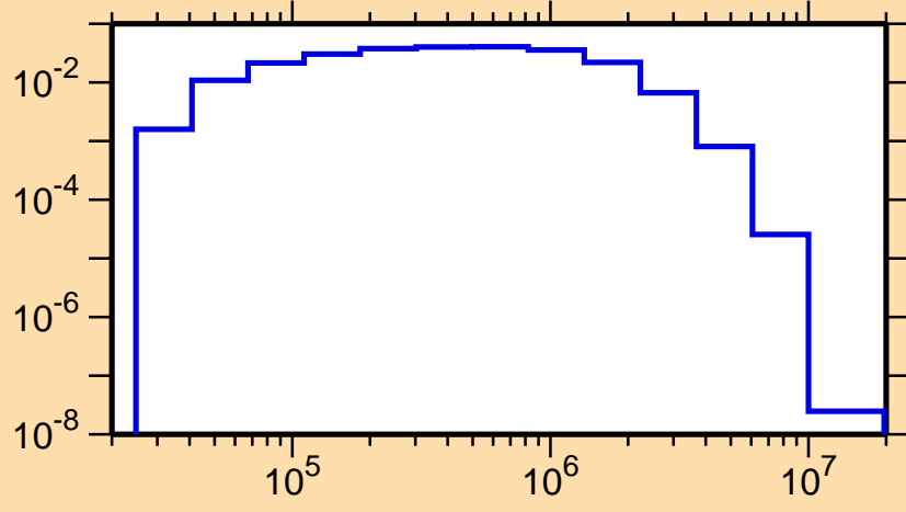
\sigma vs. E for ^{127}\text{Ce}(n,n_3)
