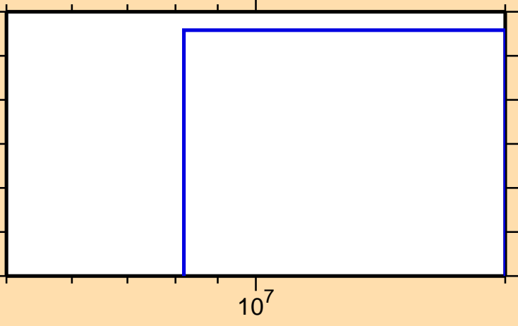
\sigma vs. E for ^{127}\text{Ce}(\text{mt117})
