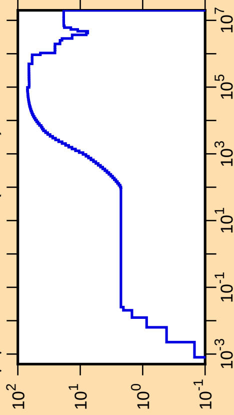
\Delta\mu/\mu vs. E for ^{128}\text{Ce}(\text{mt251})
