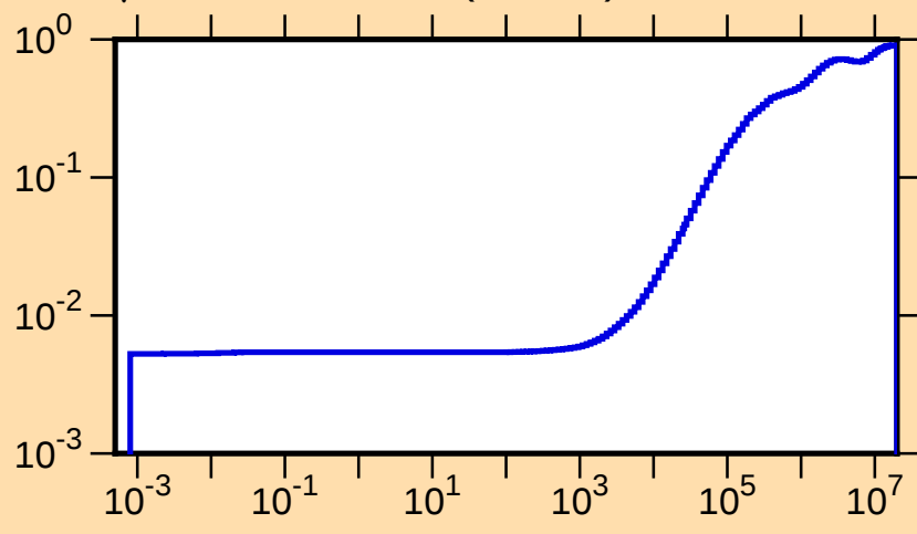
\mu vs. E for ^{128}\text{Ce}(\text{mt251})
