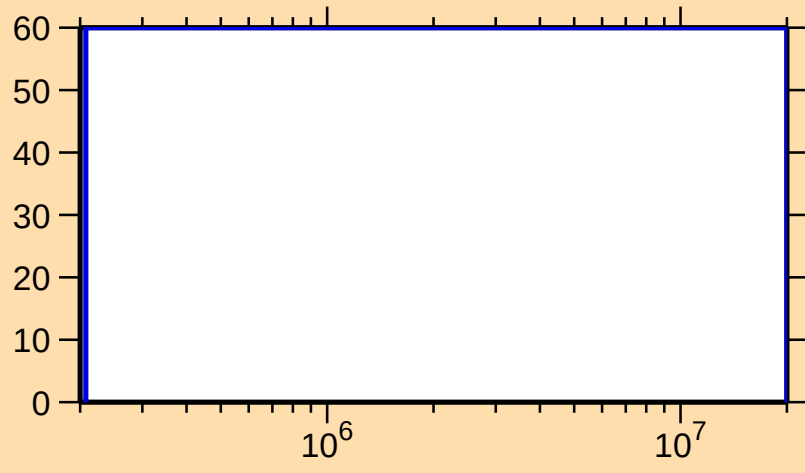
\Delta\sigma/\sigma vs. E for ^{128}\text{Ce}(n,n_1)
