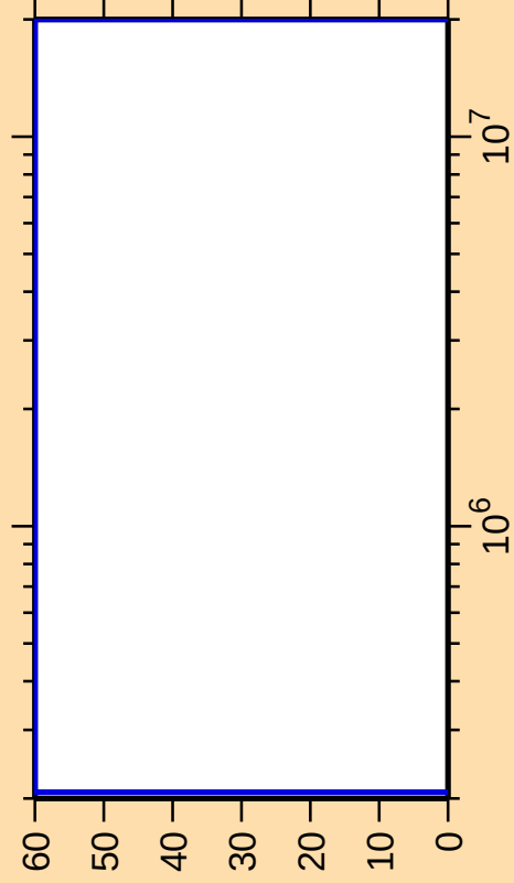
\Delta\sigma/\sigma vs. E for ^{128}\text{Ce}(n,\text{inel.})
