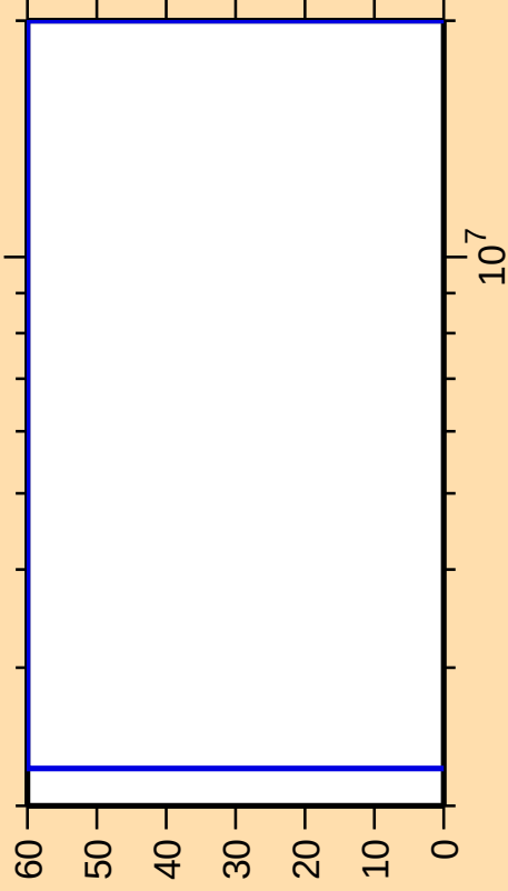
\Delta\sigma/\sigma vs. E for ^{128}\text{Ce}(n,n\text{cont.})
