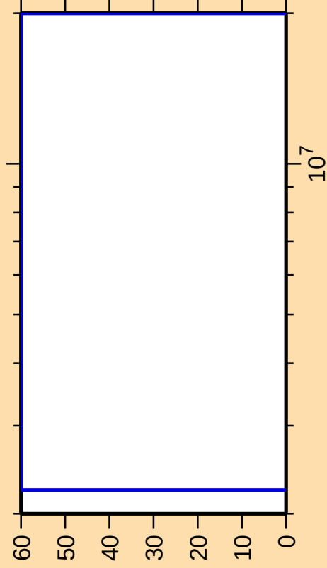
\Delta\sigma/\sigma vs. E for ^{128}\text{Ce}(n,\alpha)
