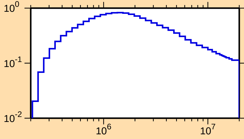
\sigma vs. E for ^{128}\text{Ce}(n,n_1)
