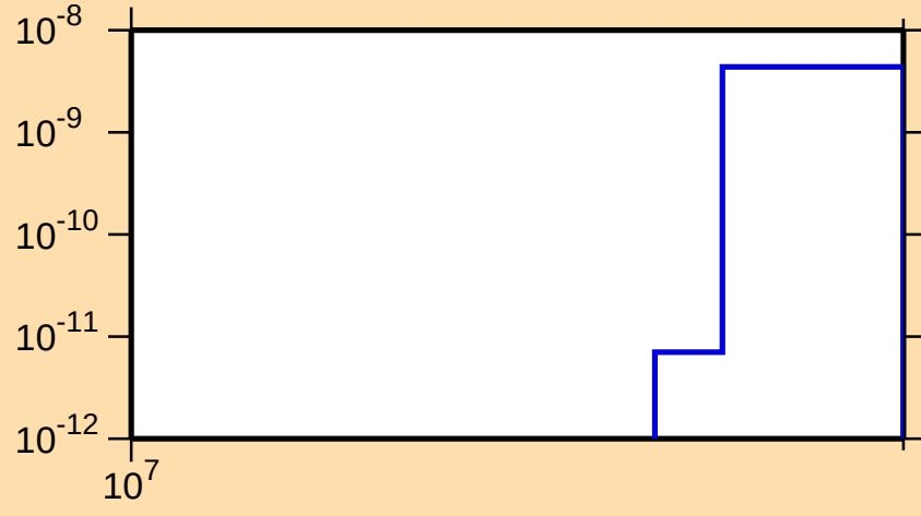
\sigma vs. E for ^{128}\text{Ce}(n,\text{pt})
