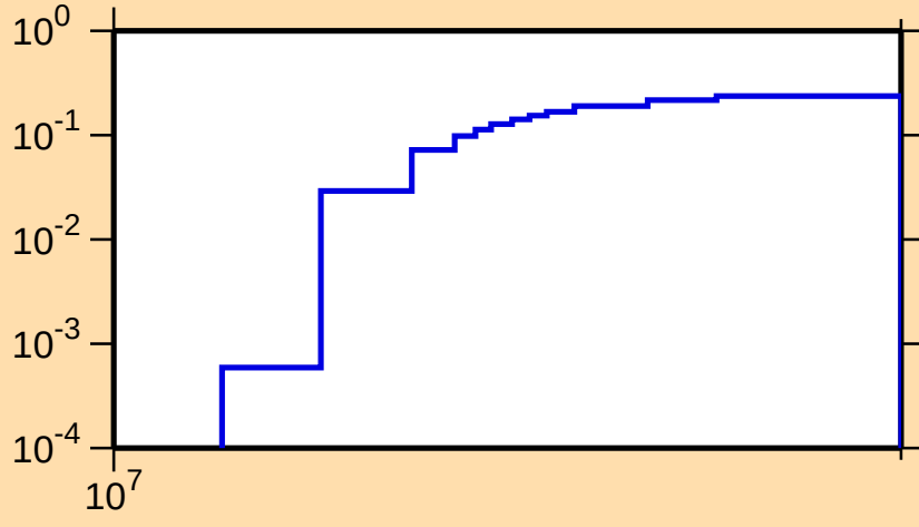
\sigma vs. E for ^{128}\text{Ce}(n,2n)
