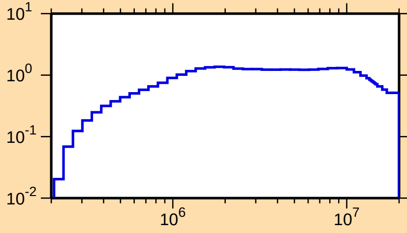
\sigma vs. E for ^{128}\text{Ce}(n,\text{inel.})
