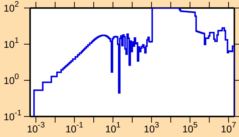
\Delta\sigma/\sigma vs. E for ^{128}\text{Ce}(n,\text{tot.})
