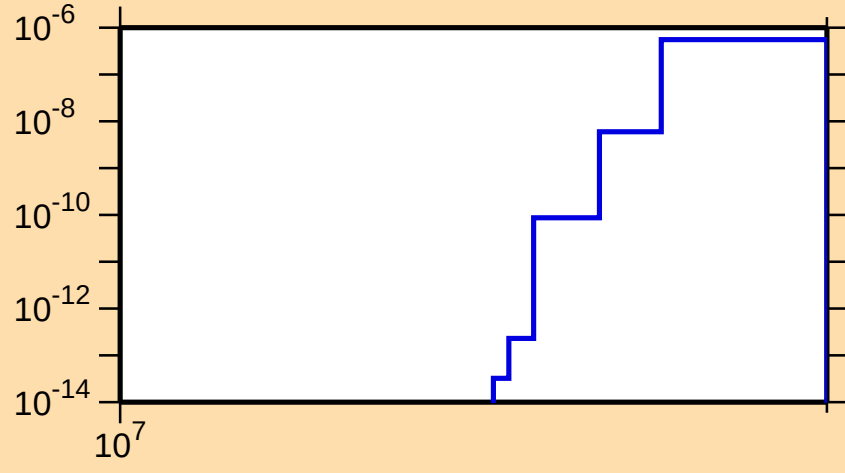
\sigma vs. E for ^{128}\text{Ce}(n,2n\alpha)
