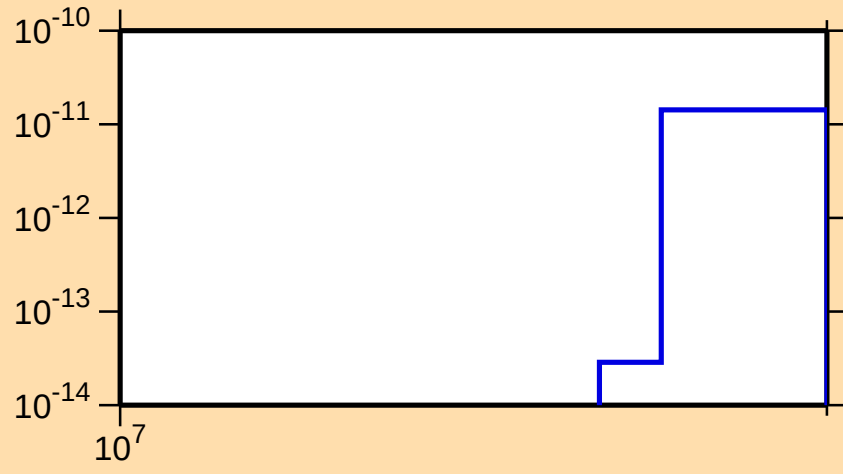
\sigma vs. E for ^{128}\text{Ce} (mt 34)
