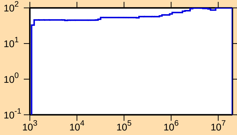
\Delta\sigma/\sigma vs. E for ^{128}\text{Ce}(n,\gamma)
