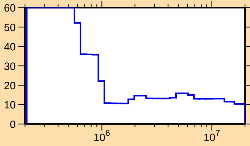
\Delta\sigma/\sigma vs. E for ^{128}\text{Ce}(n,\text{nonel.})
