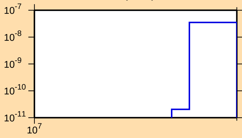
\sigma vs. E for ^{128}\text{Ce}(n,\text{nd})
