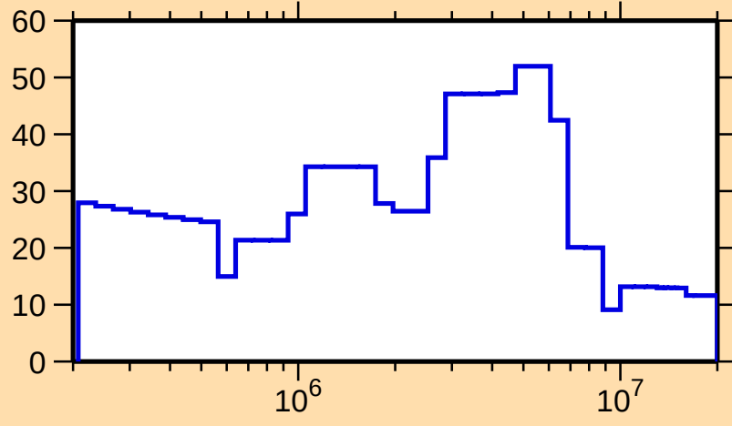
\Delta\sigma/\sigma vs. E for ^{128}\text{Ce}(n,\text{el.})
