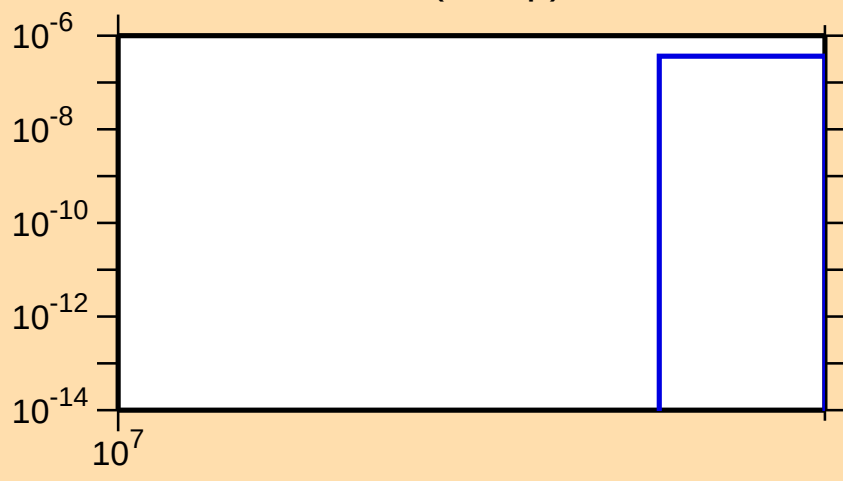
\sigma vs. E for ^{128}\text{Ce}(n,2np)
