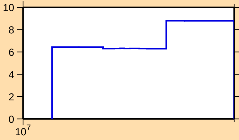
\Delta\sigma/\sigma vs. E for ^{128}\text{Ce}(n,\text{tot.})
