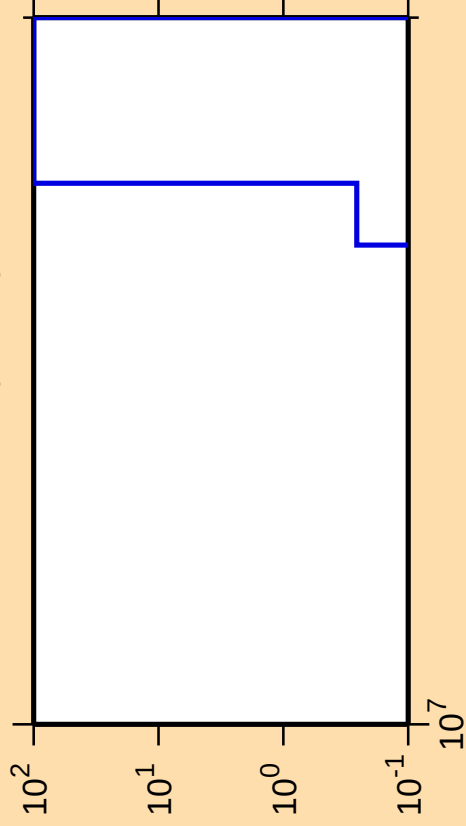
\Delta\sigma/\sigma vs. E for ^{128}\text{Ce} (mt 34)
