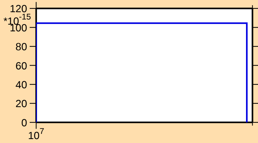
\sigma vs. E for ^{128}\text{Ce} (mt 34)
