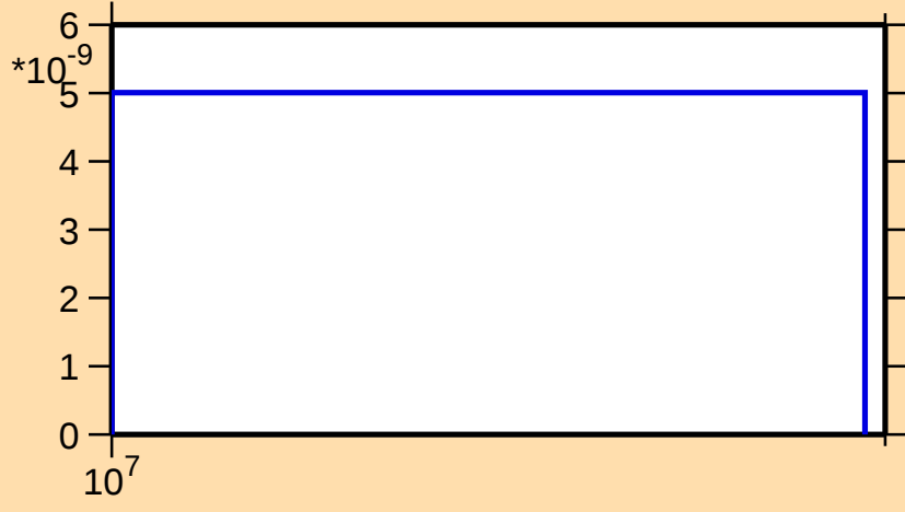
\sigma vs. E for ^{128}\text{Ce}(n,2n\alpha)
