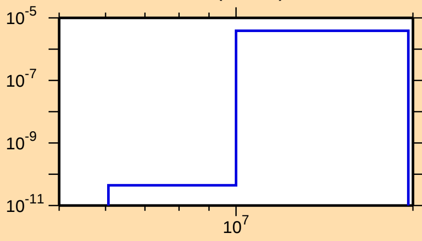
\sigma vs. E for ^{128}\text{Ce}(n,\text{He}3)
