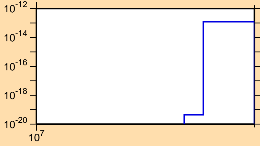
\sigma vs. E for ^{129}\text{Ce}(n,nt)
