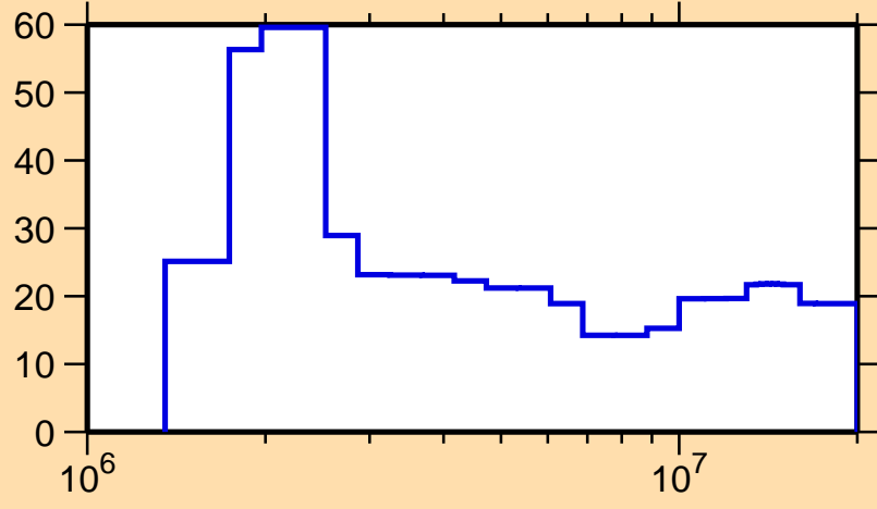
\Delta\sigma/\sigma vs. E for ^{129}\text{Ce}(n,n\text{cont.})
