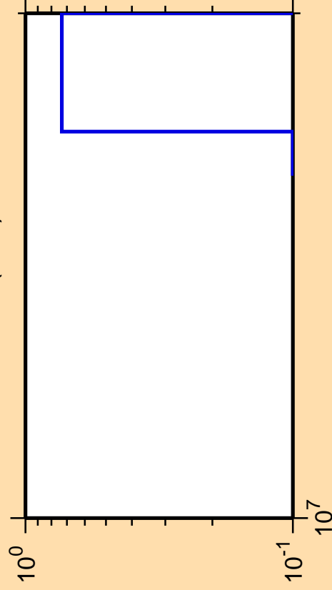
\Delta\sigma/\sigma vs. E for ^{129}\text{Ce}(n,nt)
