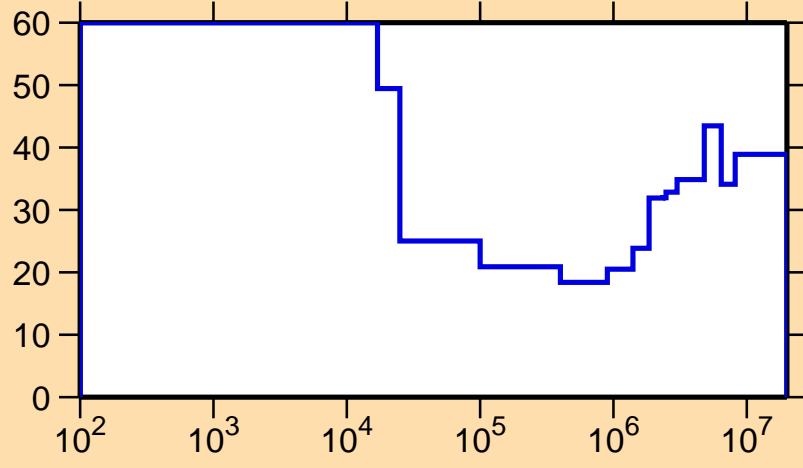
\Delta\sigma/\sigma vs. E for ^{129}\text{Ce}(n,\gamma)
