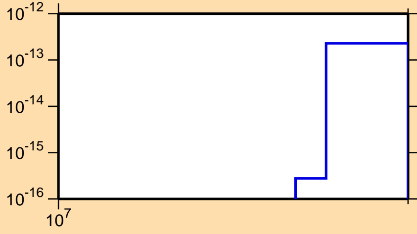
\sigma vs. E for ^{130}\text{Ce}(n,nt)
