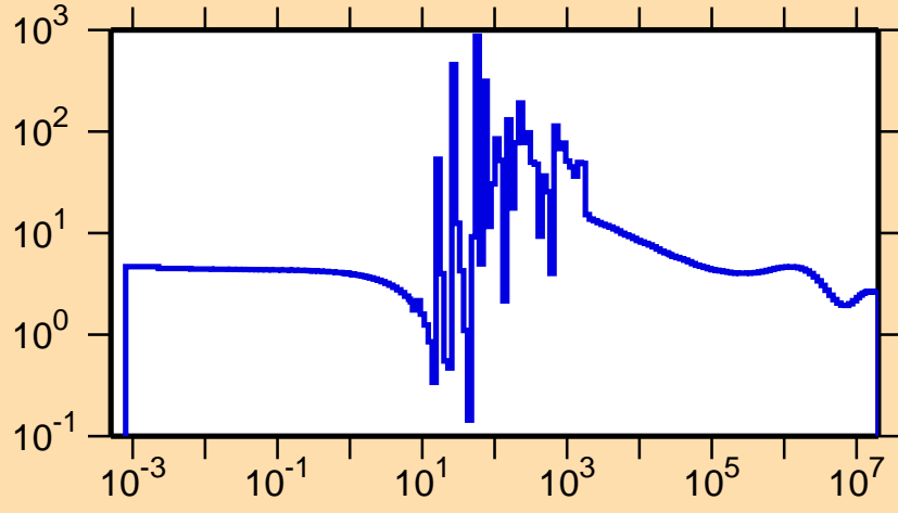
\sigma vs. E for ^{130}\text{Ce}(n,\text{el.})
