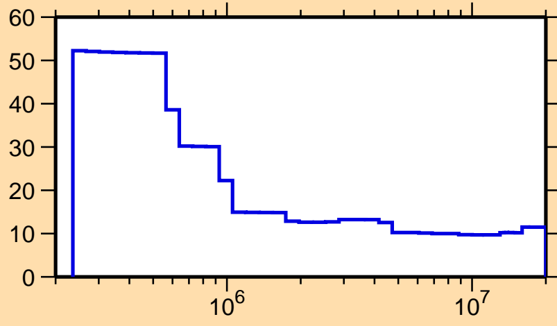
\Delta\sigma/\sigma vs. E for ^{130}\text{Ce}(n,\text{nonel.})
