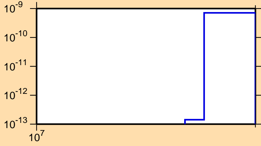
\sigma vs. E for ^{130}\text{Ce}(n,\text{pt})
