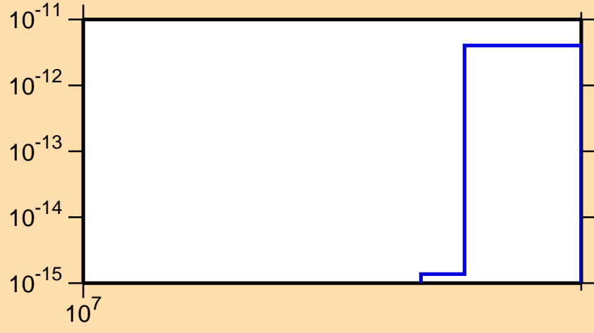
\sigma vs. E for ^{130}\text{Ce} (mt 34)
