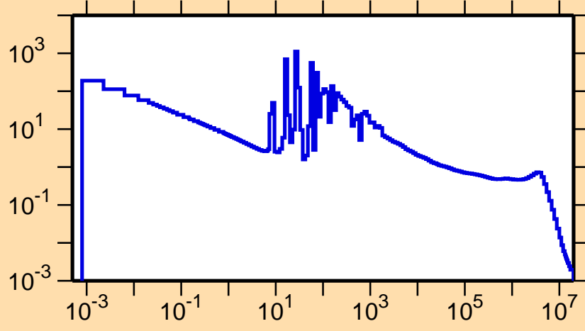
\sigma vs. E for ^{130}\text{Ce}(n,\gamma)
