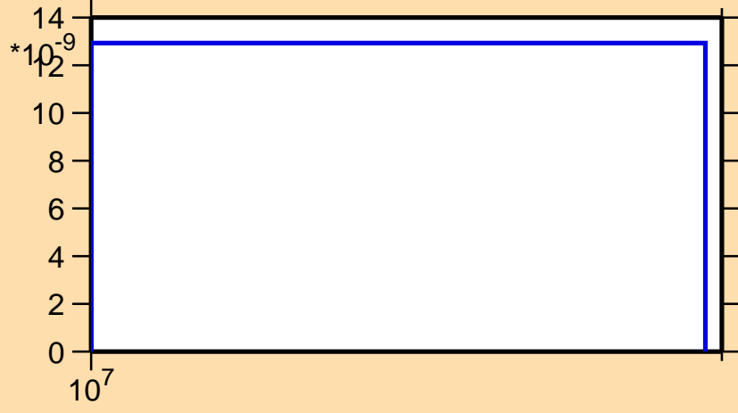
\sigma vs. E for ^{130}\text{Ce} (mt 45)
