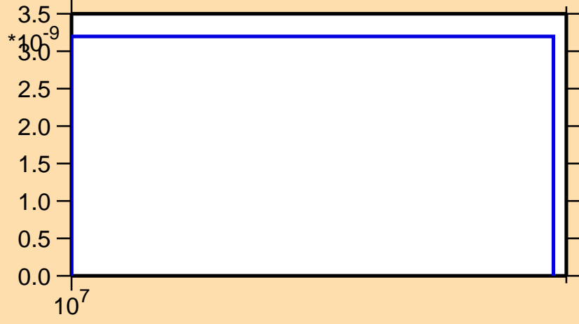
\sigma vs. E for ^{130}\text{Ce}(n,2np)
