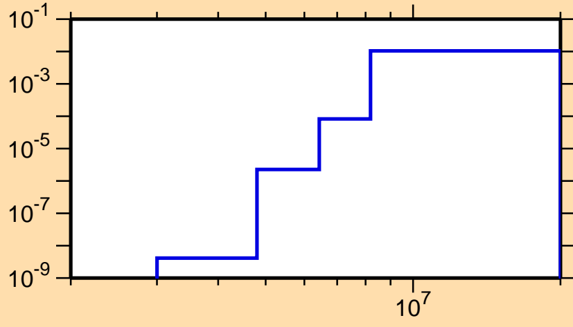
\sigma vs. E for ^{130}\text{Ce}(n,n\alpha)
