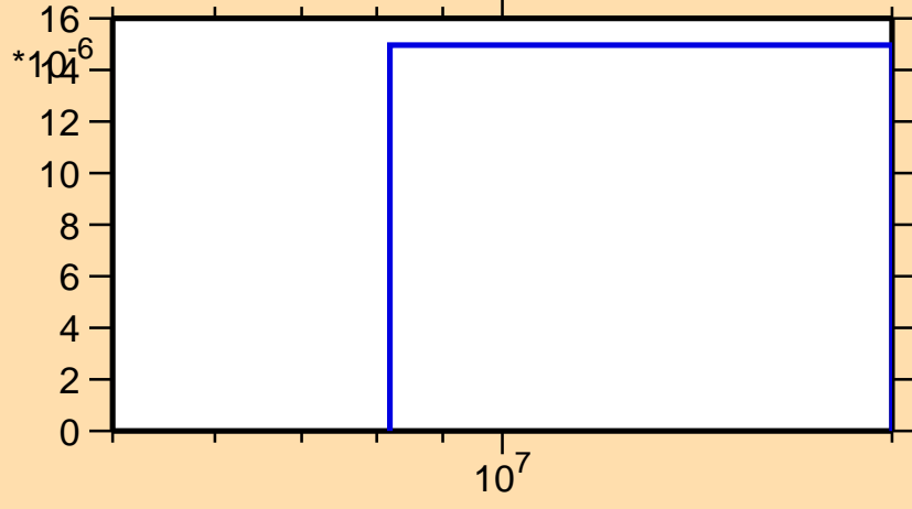
\sigma vs. E for ^{130}\text{Ce}(n,t)
