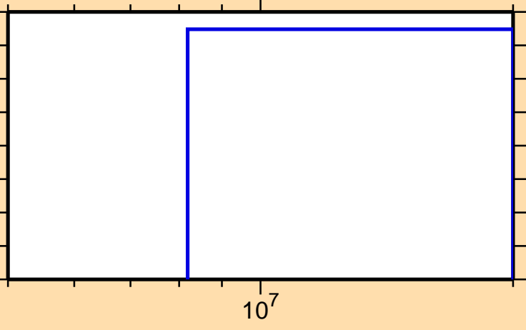
\sigma vs. E for ^{130}\text{Ce}(n,t)
