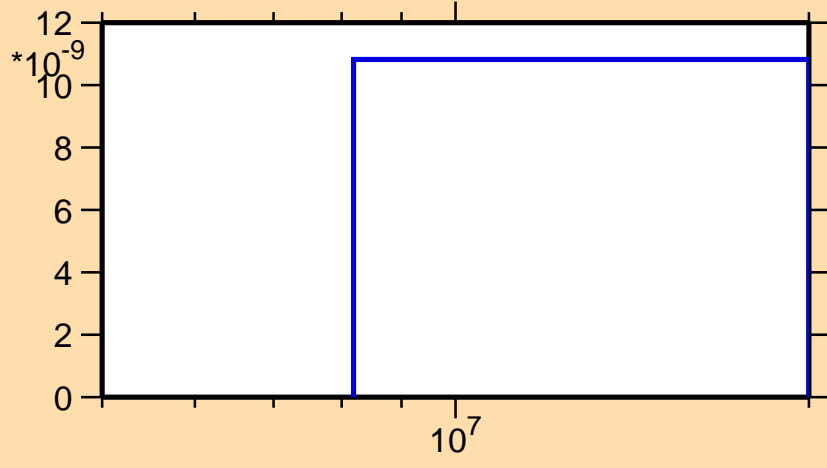
\sigma vs. E for ^{130}\text{Ce}(\text{mt } 45)
