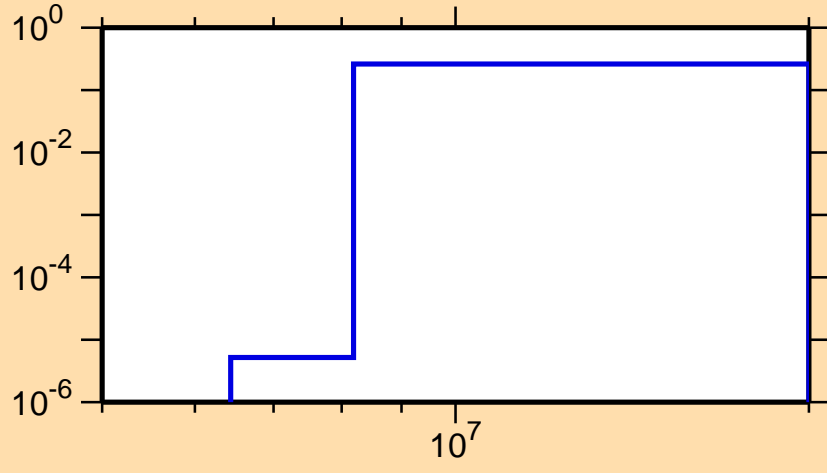
\sigma vs. E for ^{130}\text{Ce}(n,np)
