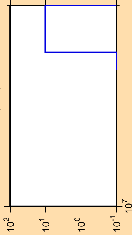
\Delta\sigma/\sigma vs. E for ^{131}\text{Ce}(n,nt)
