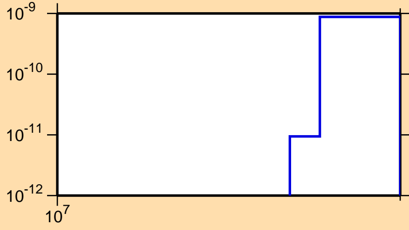
\sigma vs. E for ^{131}\text{Ce} (mt 34)
