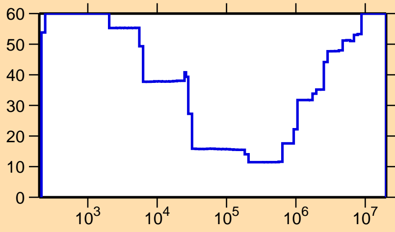
\Delta\sigma/\sigma vs. E for ^{131}\text{Ce}(n,\gamma)
