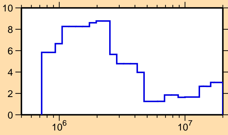
\Delta\sigma/\sigma vs. E for ^{131}\text{Ce}(n,\text{tot.})
