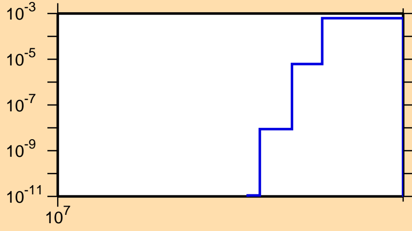
\sigma vs. E for ^{131}\text{Ce}(n,2np)
