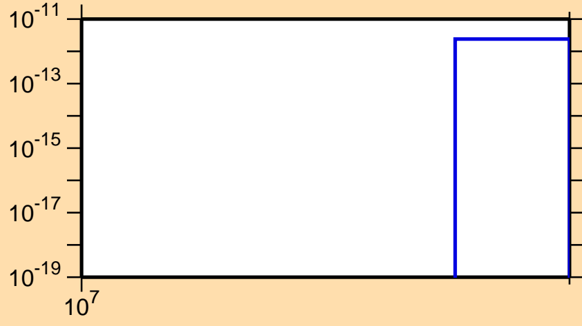
\sigma vs. E for ^{131}\text{Ce}(n,nt)
