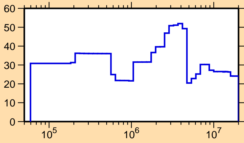
\Delta\sigma/\sigma vs. E for ^{131}\text{Ce}(n,n_1)
