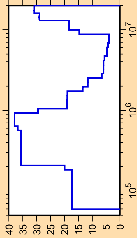
\Delta\sigma/\sigma vs. E for ^{131}\text{Ce}(n,\text{inel.})
