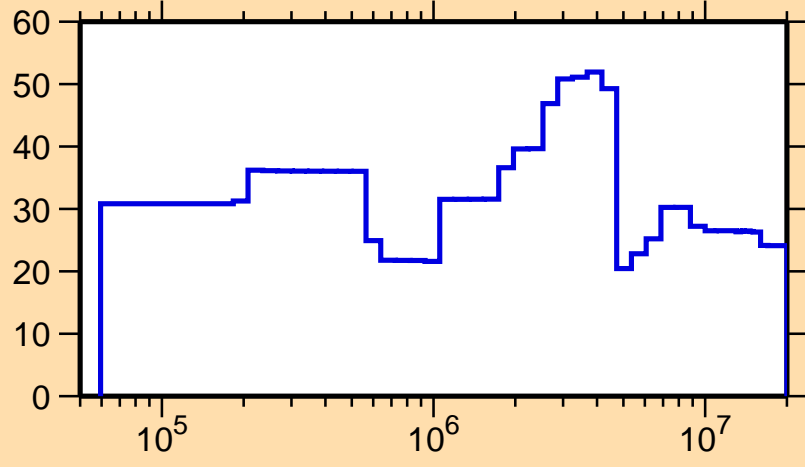
\Delta\sigma/\sigma vs. E for ^{131}\text{Ce}(n,n_1)
