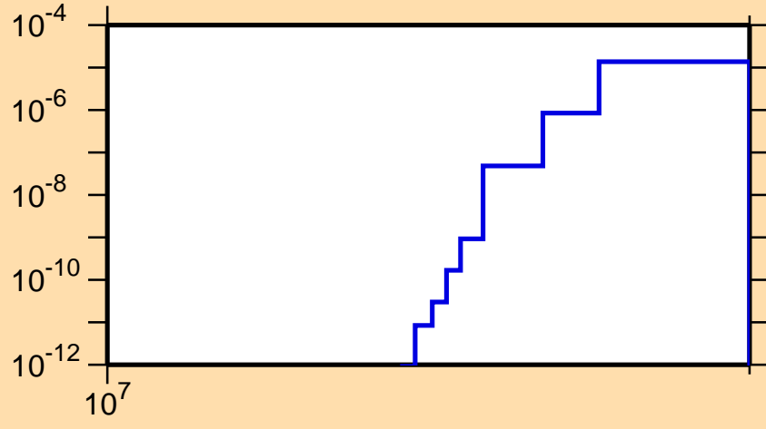
\sigma vs. E for ^{131}\text{Ce}(n,\text{nd})
