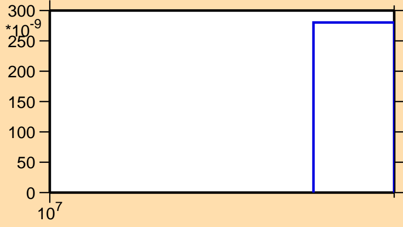
\sigma vs. E for ^{131}\text{Ce}(n,3n)
