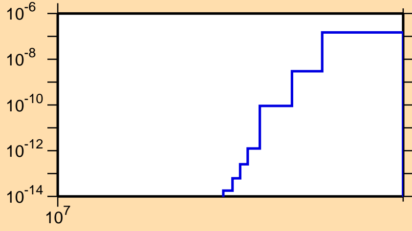
\sigma vs. E for ^{131}\text{Ce}(n,\text{pt})
