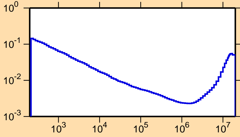
\sigma vs. E for ^{131}\text{Ce}(n,\alpha)
