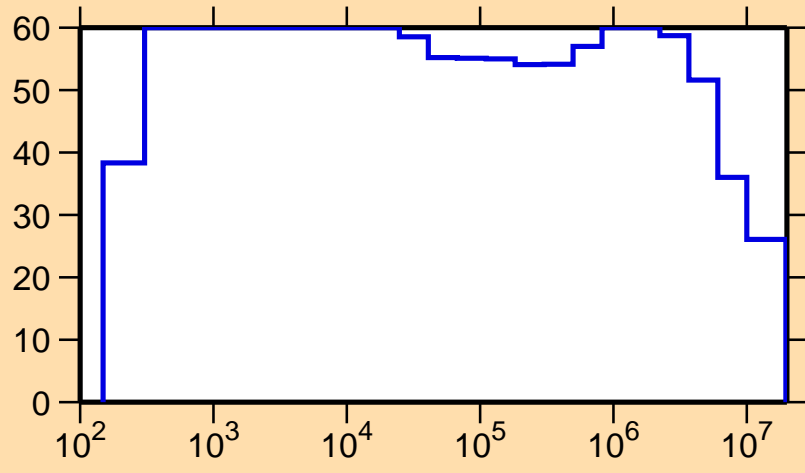
\Delta\sigma/\sigma vs. E for ^{131}\text{Ce}(n,p)
