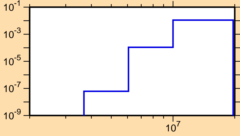
\sigma vs. E for ^{131}\text{Ce}(n,n\alpha)
