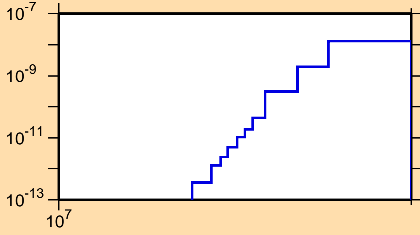
\sigma vs. E for ^{131}\text{Ce}(\text{mt117})
