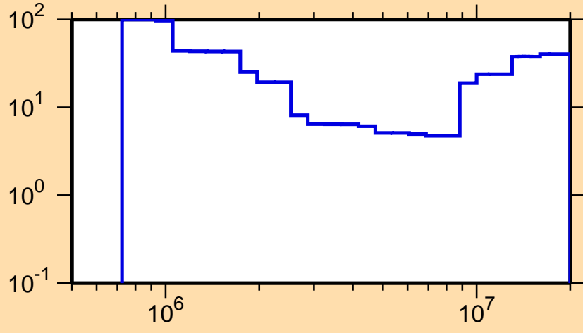
\Delta\sigma/\sigma vs. E for ^{131}\text{Ce}(n,n\text{cont.})
