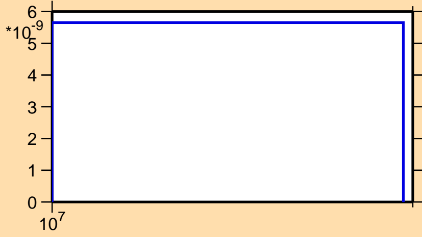
\sigma vs. E for ^{131}\text{Ce} (mt 45)
