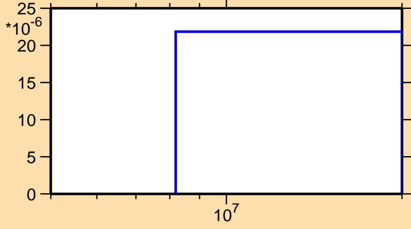
\sigma vs. E for ^{131}\text{Ce}(n,2np)
