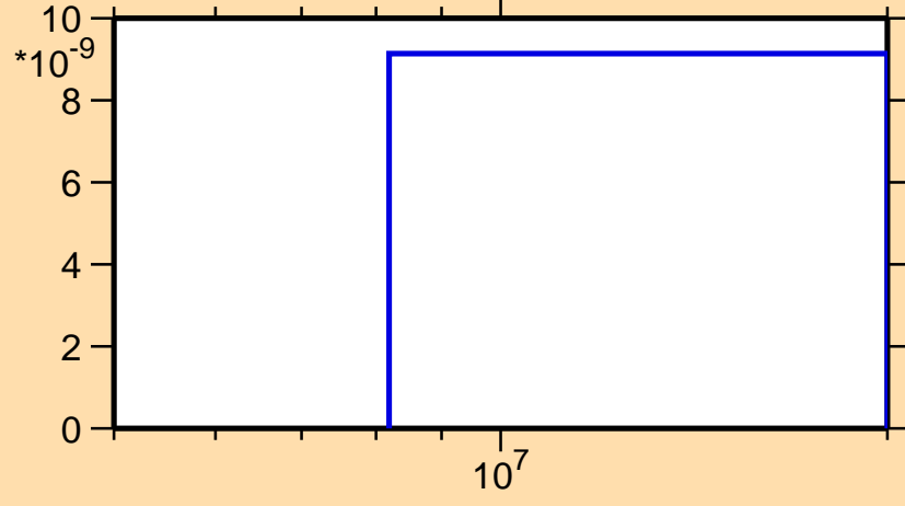
\sigma vs. E for ^{131}\text{Ce}(n,3n)
