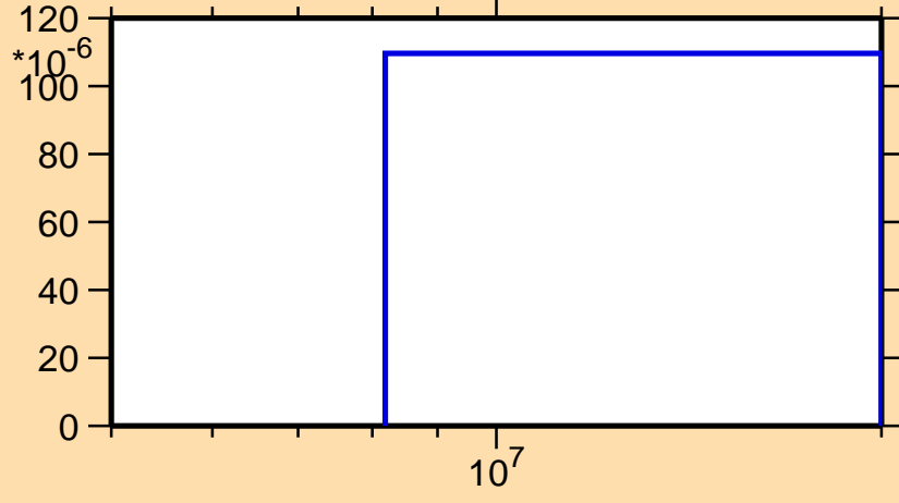
\sigma vs. E for ^{131}\text{Ce}(n,t)
