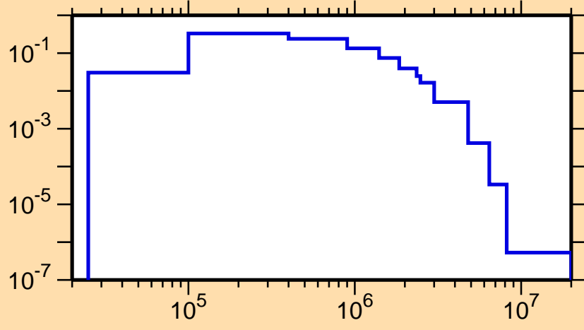
\sigma vs. E for ^{131}\text{Ce}(n,n_2)
