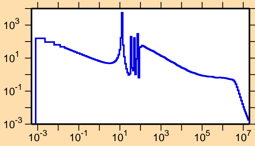
\sigma vs. E for ^{132}\text{Ce}(n,\gamma)
