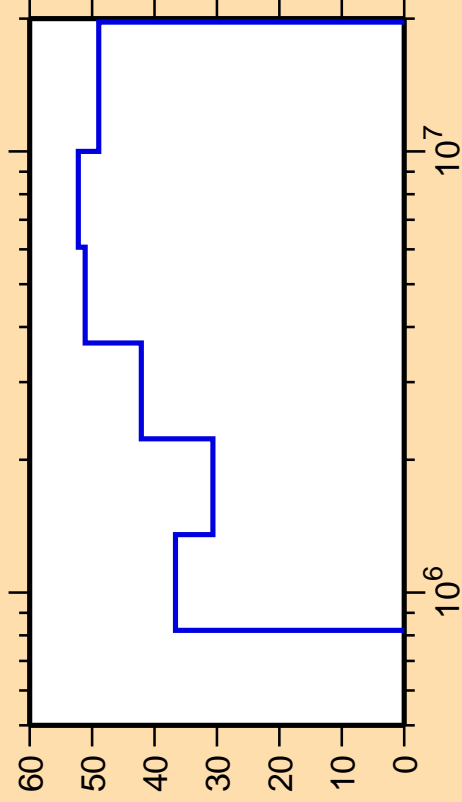
\Delta\sigma/\sigma vs. E for ^{132}\text{Ce}(n,n_3)
