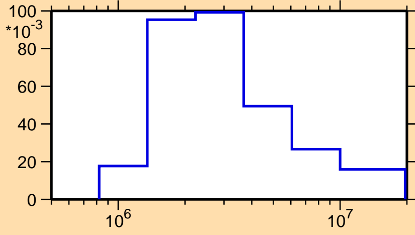
\sigma vs. E for ^{132}\text{Ce}(n,n_3)
