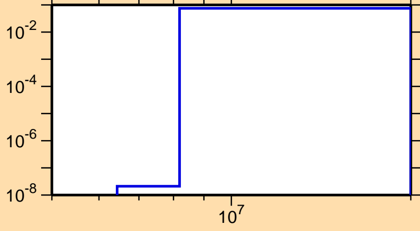
\sigma vs. E for ^{132}\text{Ce}(n,np)
