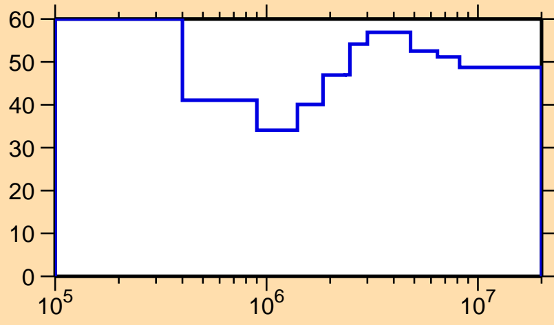
\Delta\sigma/\sigma vs. E for ^{132}\text{Ce}(n,n_1)
