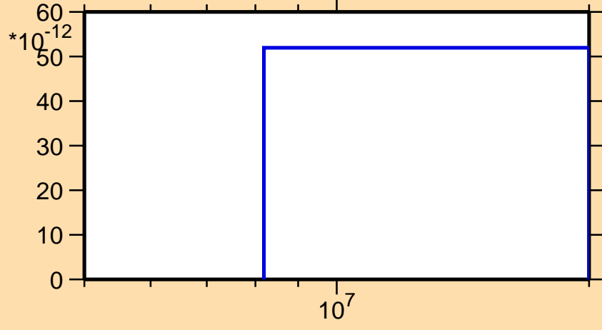
\sigma vs. E for ^{132}\text{Ce}(\text{mt } 45)
