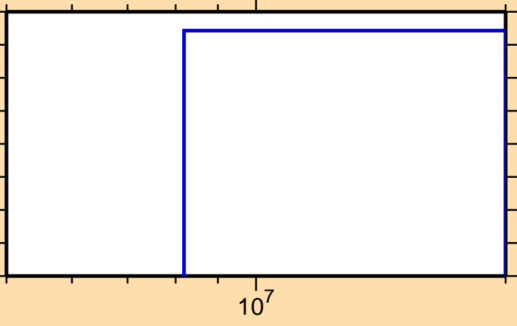
\sigma vs. E for ^{132}\text{Ce}(n,\text{nd})
