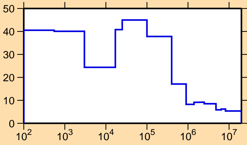
\Delta\sigma/\sigma vs. E for ^{132}\text{Ce}(n,\text{nonel.})
