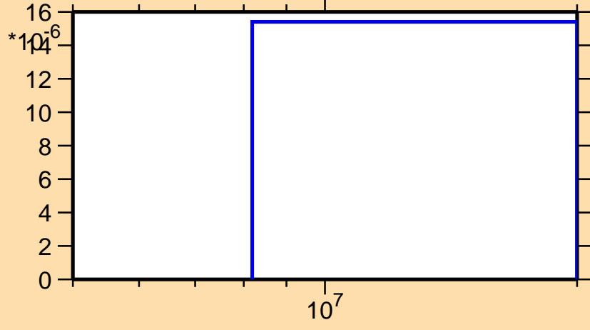
\sigma vs. E for ^{132}\text{Ce}(n,t)
