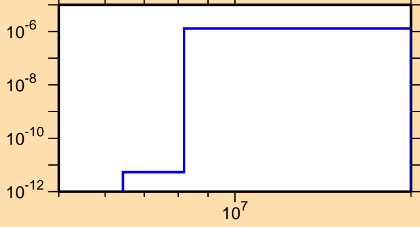
\sigma vs. E for ^{132}\text{Ce}(n,p\alpha)
