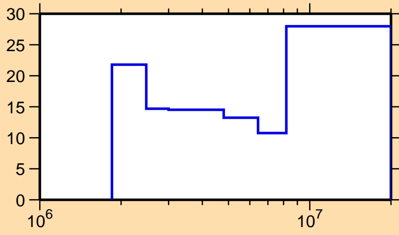
\Delta\sigma/\sigma vs. E for ^{132}\text{Ce}(n,n\text{cont.})
