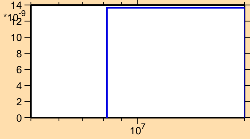
\sigma vs. E for ^{132}\text{Ce}(n,3n)
