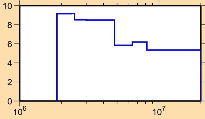
\Delta\sigma/\sigma vs. E for ^{132}\text{Ce}(n,n\text{onel.})
