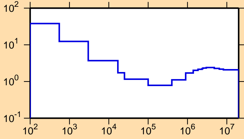
\sigma vs. E for ^{132}\text{Ce}(n,\text{nonel.})
