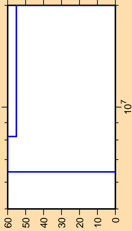
\Delta\sigma/\sigma vs. E for ^{132}\text{Ce}(n,np)
