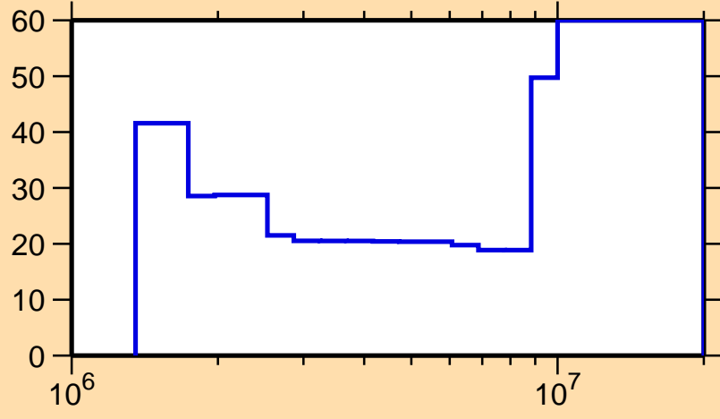
\Delta\sigma/\sigma vs. E for ^{133}\text{Ce}(n,n\text{cont.})
