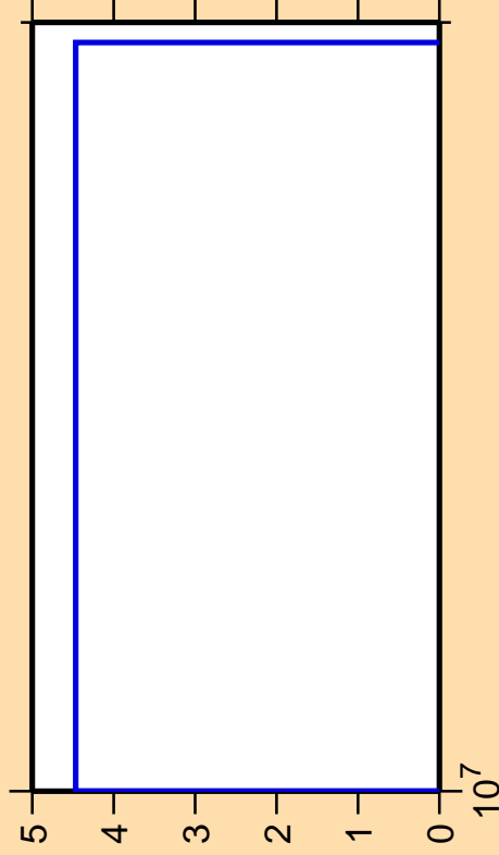
\Delta\sigma/\sigma vs. E for ^{133}\text{Ce}(\text{mt117})
