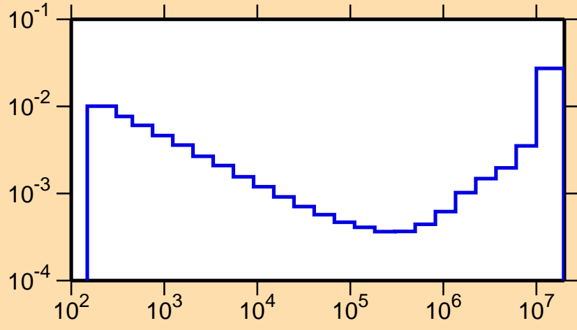
\sigma vs. E for ^{133}\text{Ce}(n,\alpha)
