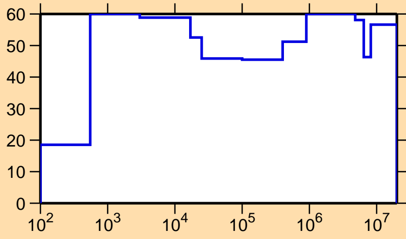
\Delta\sigma/\sigma vs. E for ^{133}\text{Ce}(n,p)
