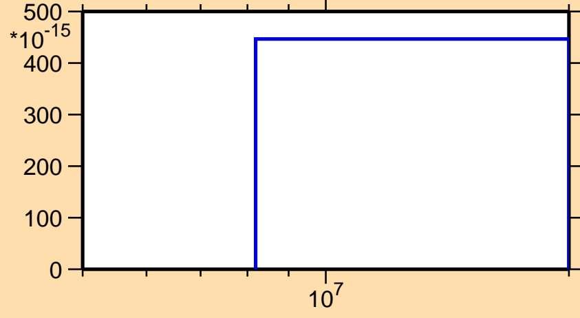
\sigma vs. E for ^{133}\text{Ce}(\text{mt } 34)
