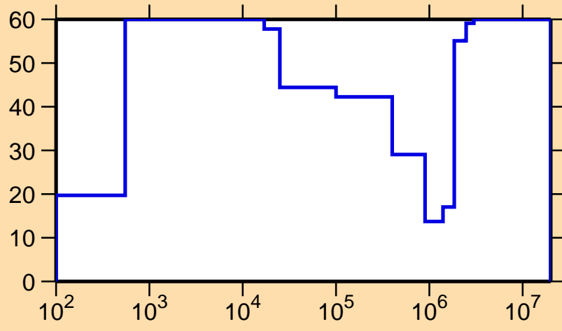
\Delta\sigma/\sigma vs. E for ^{133}\text{Ce}(n,\gamma)
