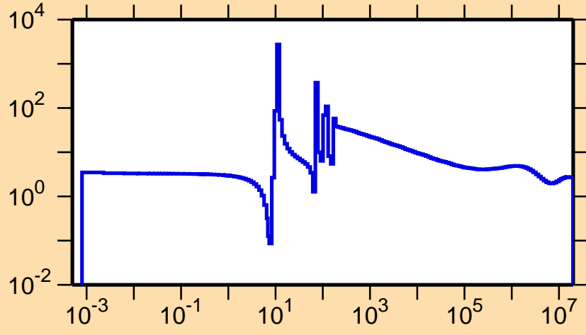
\sigma vs. E for ^{134}\text{Ce}(n,\text{el.})
