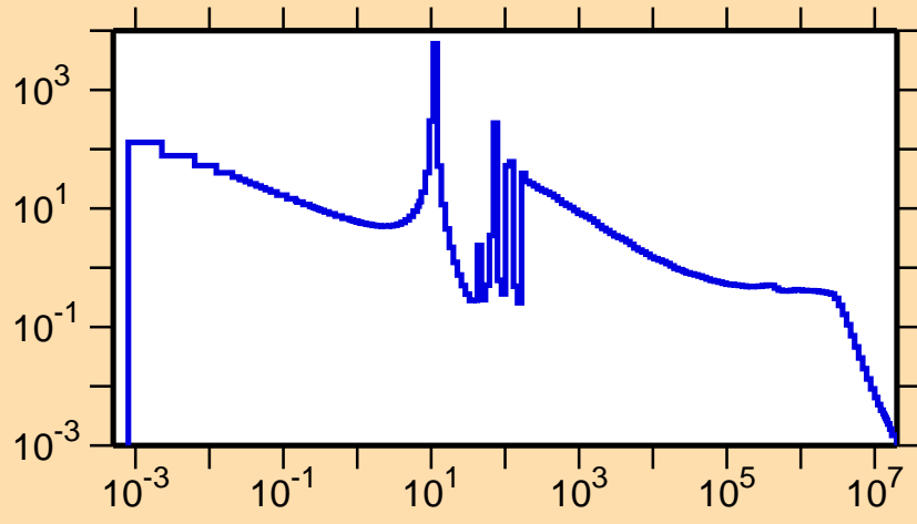
\sigma vs. E for ^{134}\text{Ce}(n,\gamma)
