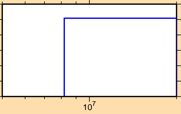
\sigma vs. E for ^{134}\text{Ce}(n,t)
