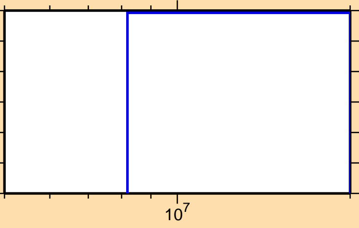
\sigma vs. E for ^{134}\text{Ce} (mt 45)
