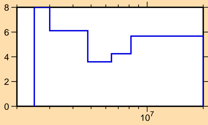
\Delta\sigma/\sigma vs. E for ^{134}\text{Ce}(n,n\text{onel.})
