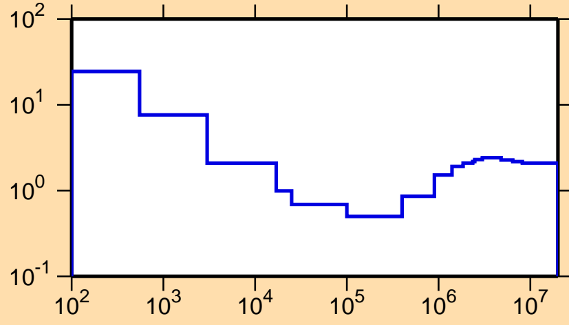
\sigma vs. E for ^{134}\text{Ce}(n,\text{nonel.})
