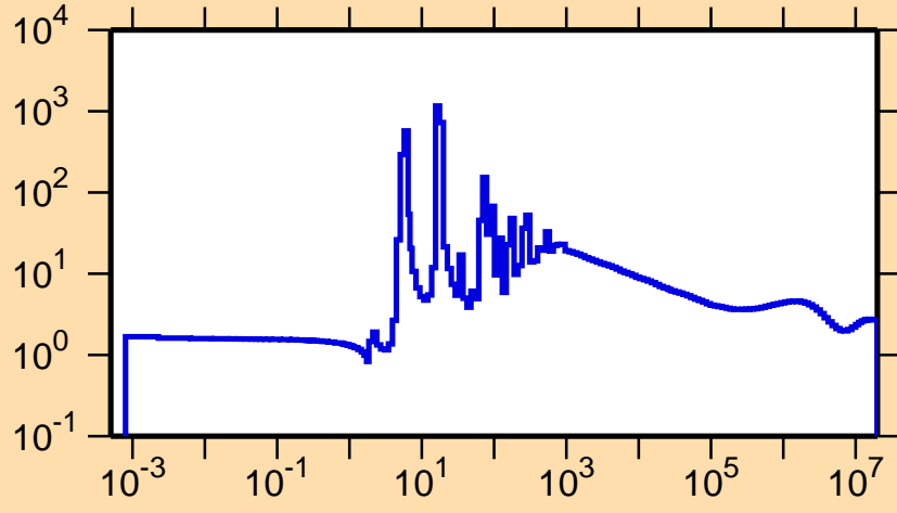
\sigma vs. E for ^{135}\text{Ce}(n,\text{el.})
