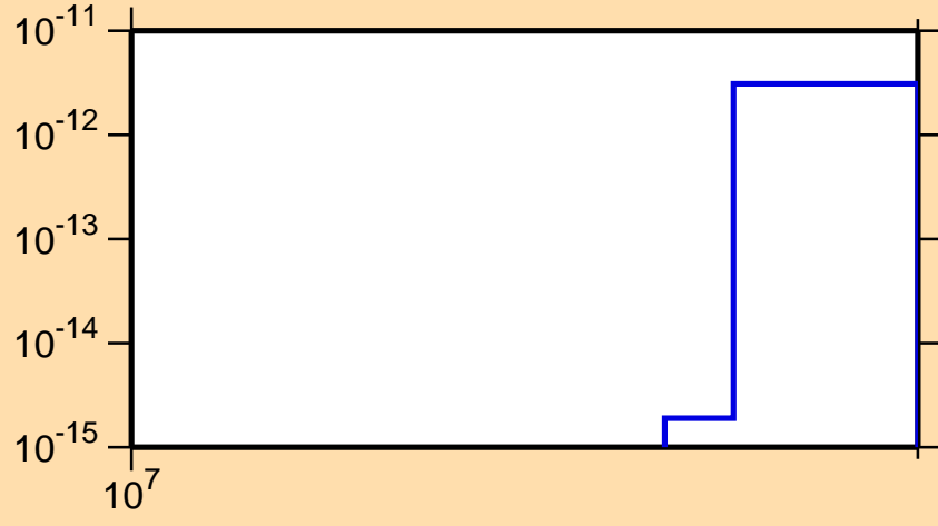
\sigma vs. E for ^{135}\text{Ce} (mt 34)
