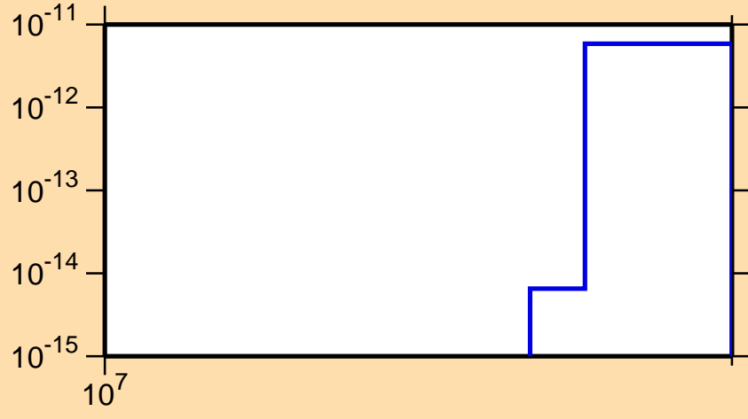
\sigma vs. E for ^{135}\text{Ce}(\text{mt } 34)
