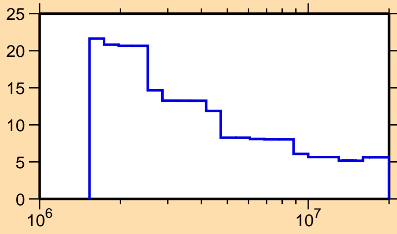
\Delta\sigma/\sigma vs. E for ^{135}\text{Ce}(n,n\text{onel.})
