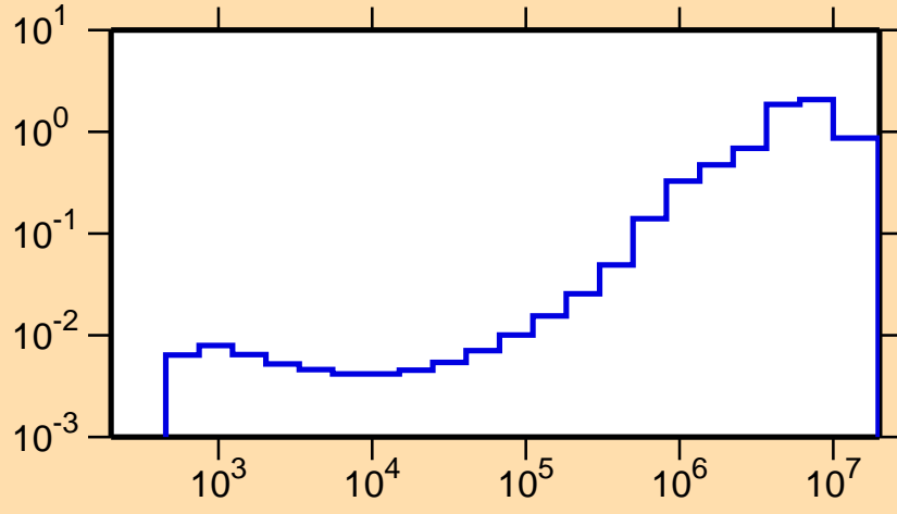
\sigma vs. E for ^{135}\text{Ce}(n,\text{inel.})
