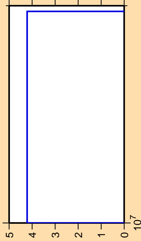
\Delta\sigma/\sigma vs. E for ^{135}\text{Ce}(n,\text{pt})
