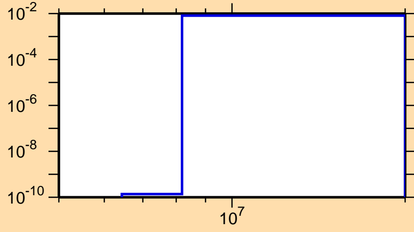
\sigma vs. E for ^{135}\text{Ce}(n,np)
