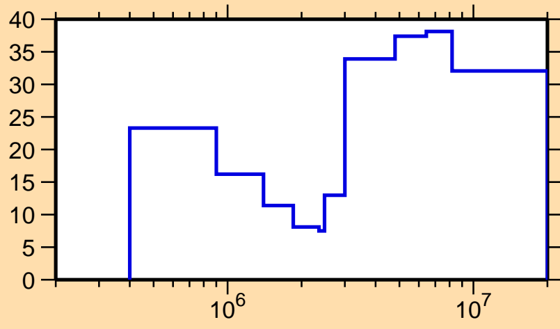
\Delta\sigma/\sigma vs. E for ^{136}\text{Ce}(n,n_1)
