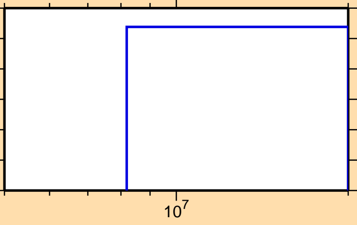
\sigma vs. E for ^{136}\text{Ce}(n,\text{He}3)
