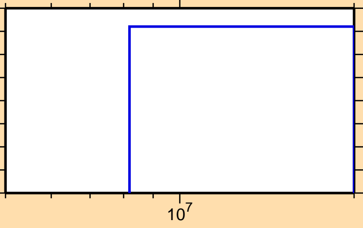
\sigma vs. E for ^{136}\text{Ce}(n,t)
