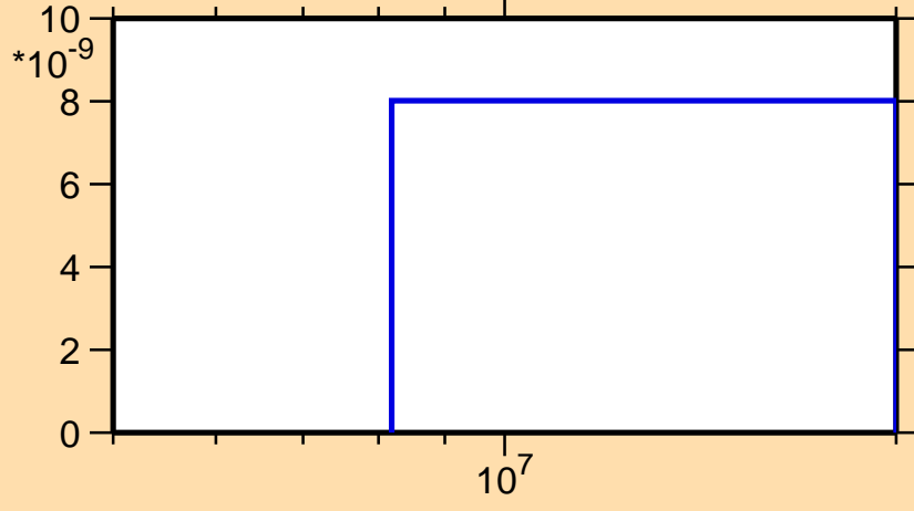
\sigma vs. E for ^{136}\text{Ce}(n,2n\alpha)
