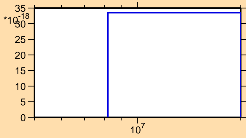
\sigma vs. E for ^{136}\text{Ce}(n,\text{pt})
