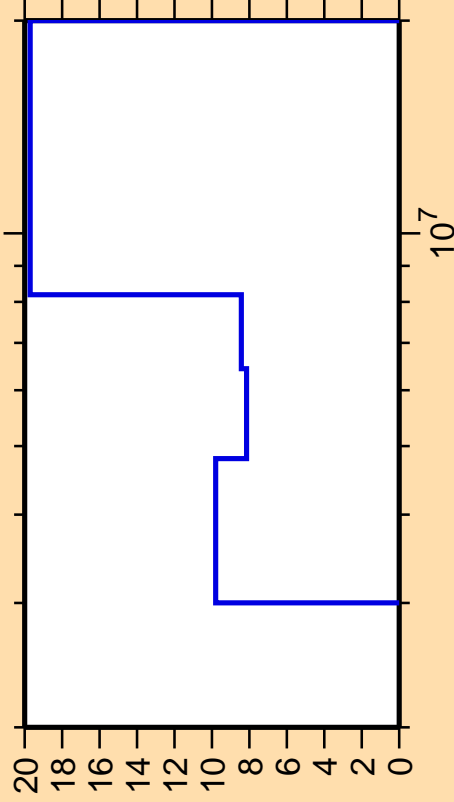
\Delta\sigma/\sigma vs. E for ^{136}\text{Ce}(n,n_{\text{cont}}) .
