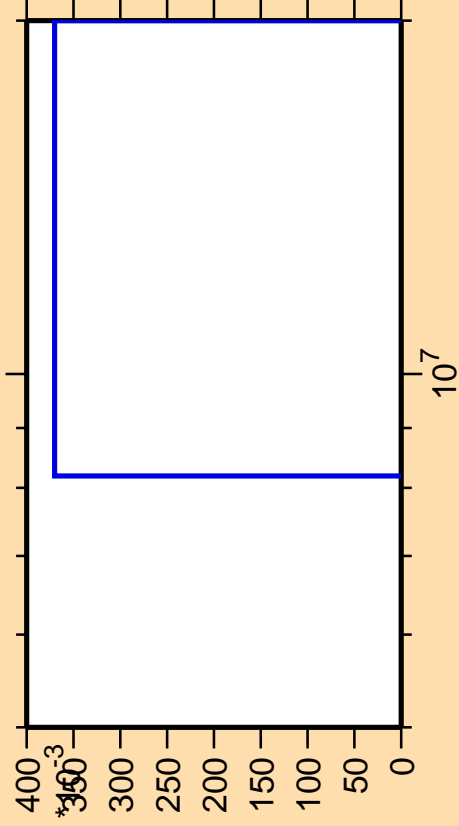
\Delta\sigma/\sigma vs. E for ^{136}\text{Ce}(\text{mt } 45)
