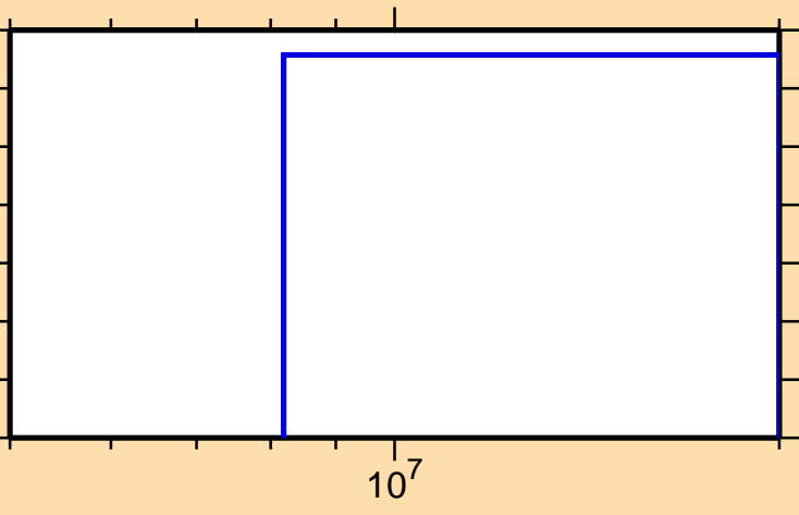
\sigma vs. E for ^{136}\text{Ce}(\text{mt } 45)
