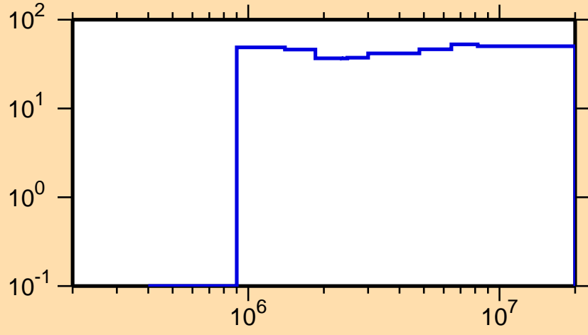
\Delta\sigma/\sigma vs. E for ^{136}\text{Ce}(n,p)
