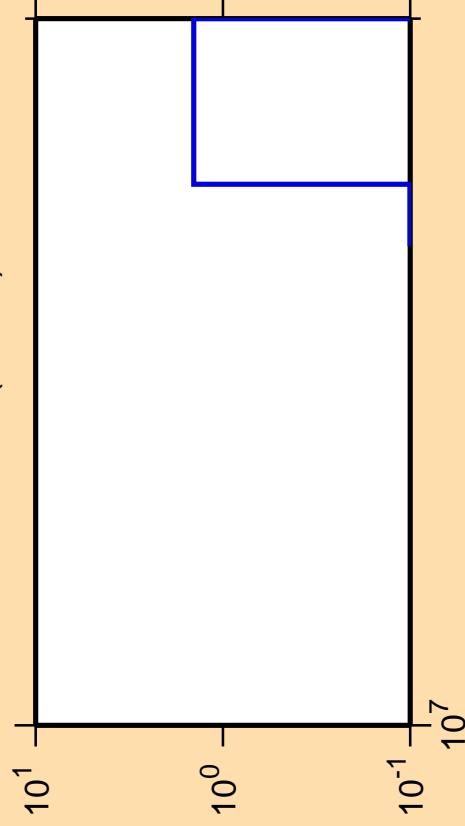
\Delta\sigma/\sigma vs. E for ^{137}\text{Ce} (mt 45)
