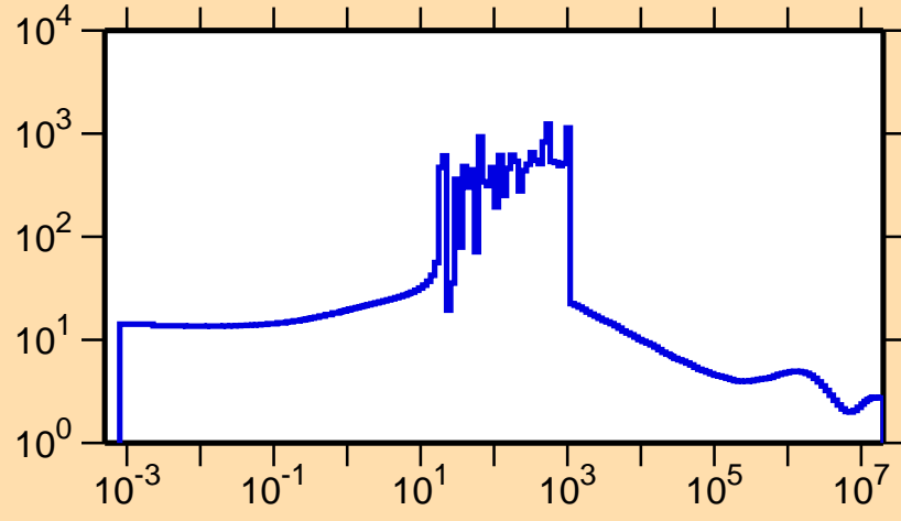
\sigma vs. E for ^{137}\text{Ce}(n,\text{el.})
