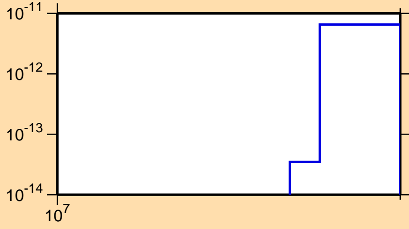
\sigma vs. E for ^{137}\text{Ce}(n,\text{pd})
