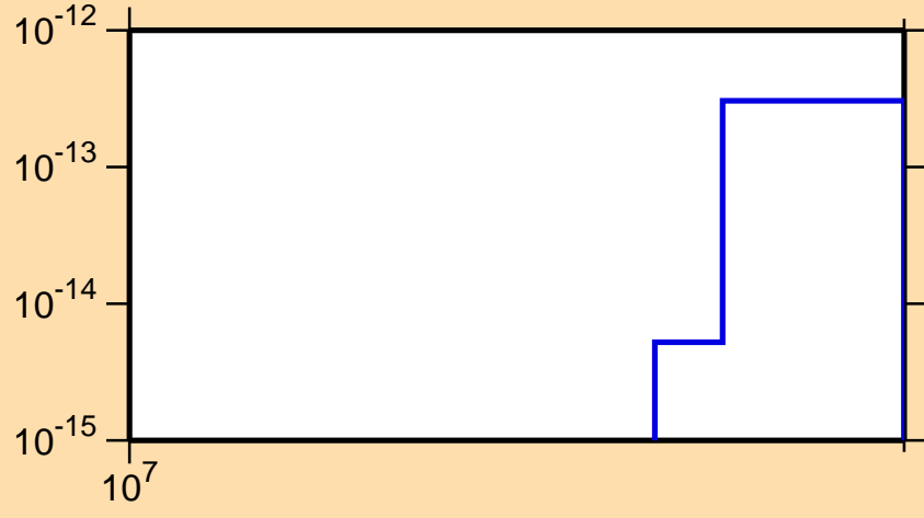
\sigma vs. E for ^{137}\text{Ce}(\text{mt117})
