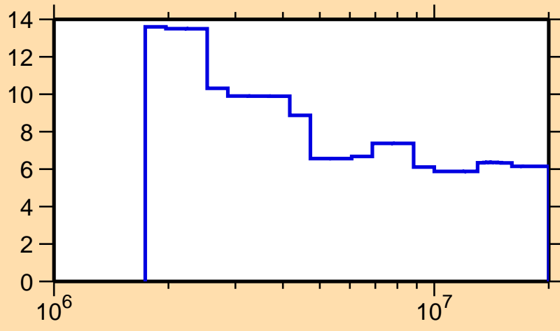
\Delta\sigma/\sigma vs. E for ^{137}\text{Ce}(n,n\text{onel.})
