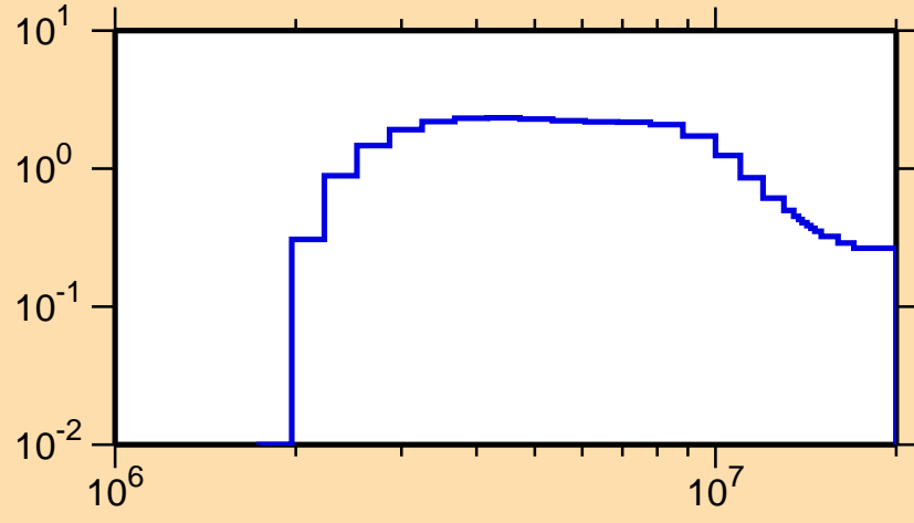
\sigma vs. E for ^{137}\text{Ce}(n,n\text{cont.})
