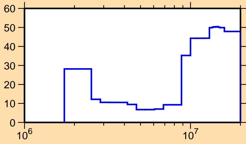
\Delta\sigma/\sigma vs. E for ^{137}\text{Ce}(n,n\text{cont.})
