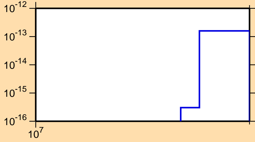
\sigma vs. E for ^{137}\text{Ce} (mt 45)
