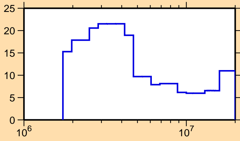
\Delta\sigma/\sigma vs. E for ^{137}\text{Ce}(n,\text{el.})
