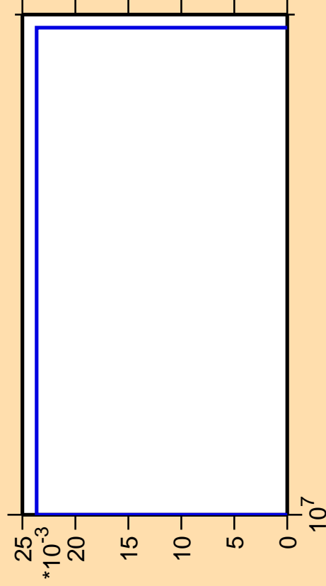
\Delta\sigma/\sigma vs. E for ^{137}\text{Ce}(\text{mt117})
