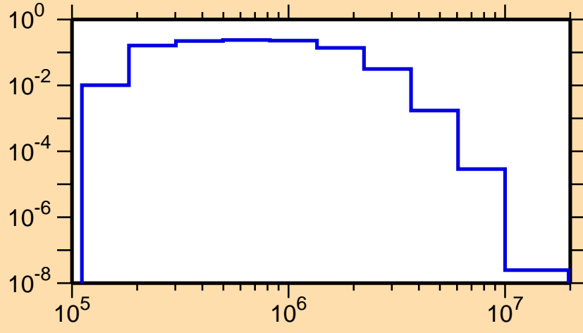
\sigma vs. E for ^{137}\text{Ce}(n,n_1)
