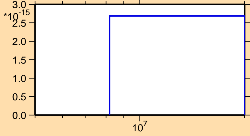
\sigma vs. E for ^{137}\text{Ce}(\text{mt117})
