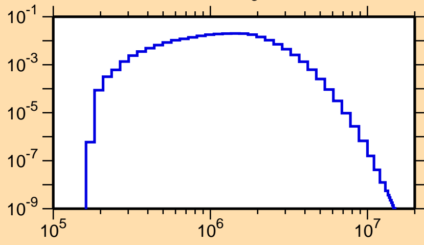
\sigma vs. E for ^{137}\text{Ce}(n,n_3)
