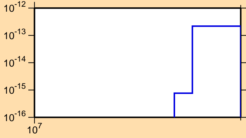
\sigma vs. E for ^{137}\text{Ce} (mt 45)
