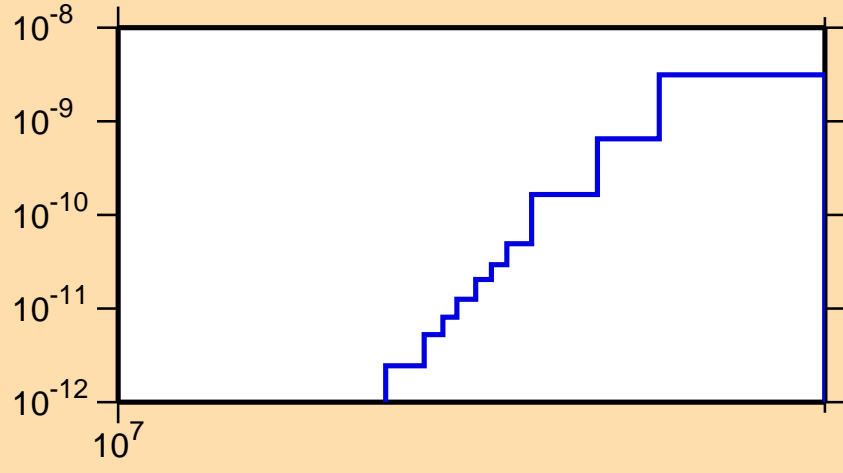
\sigma vs. E for ^{138}\text{Ce}(n,p\alpha)
