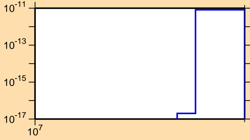
\sigma vs. E for ^{138}\text{Ce}(n,nt)
