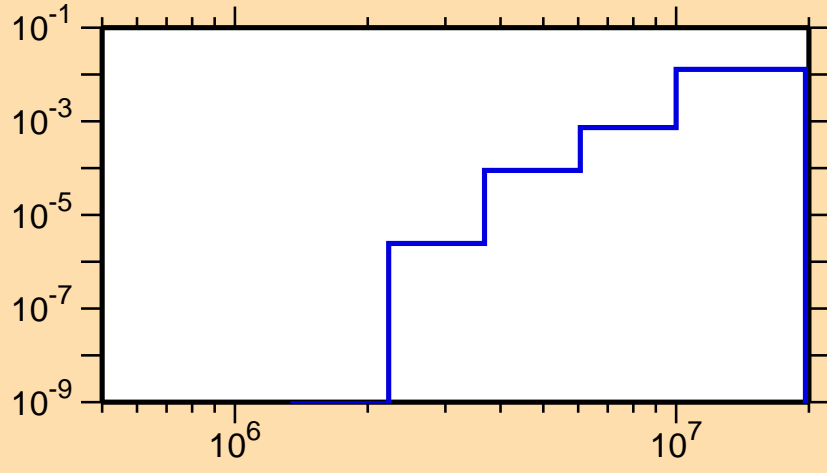
\sigma vs. E for ^{138}\text{Ce}(n,p)
